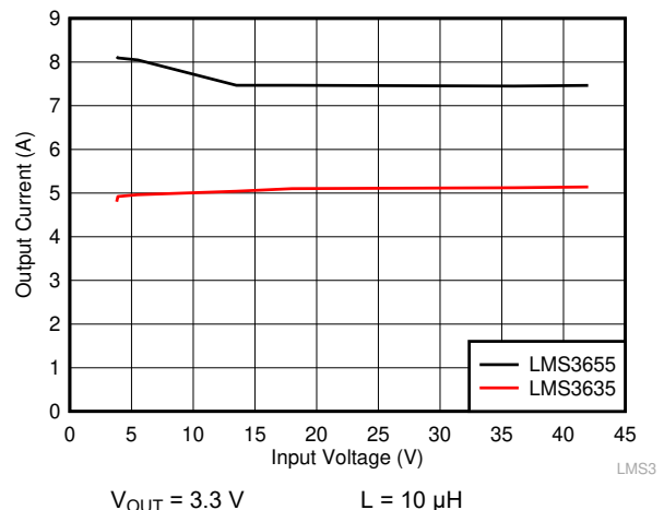
Figure 9-26. Output Current Level for Overcurrent Protection Trip
