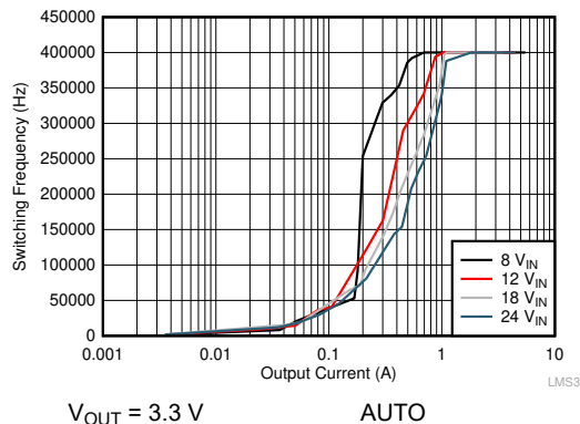
Figure 9-25. Switching Frequency vs Load Current
