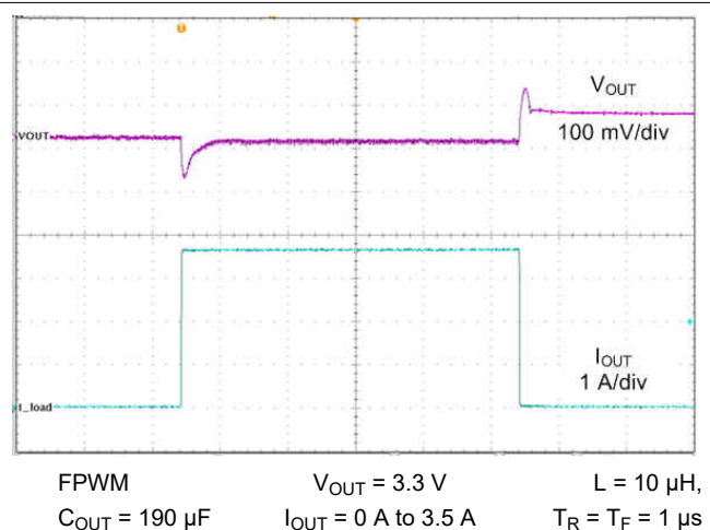
Figure 9-28. Load Transient
