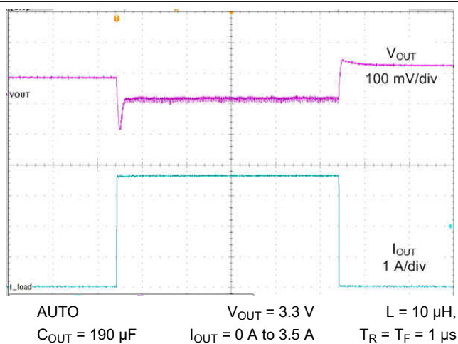
Figure 9-27. Load Transient
