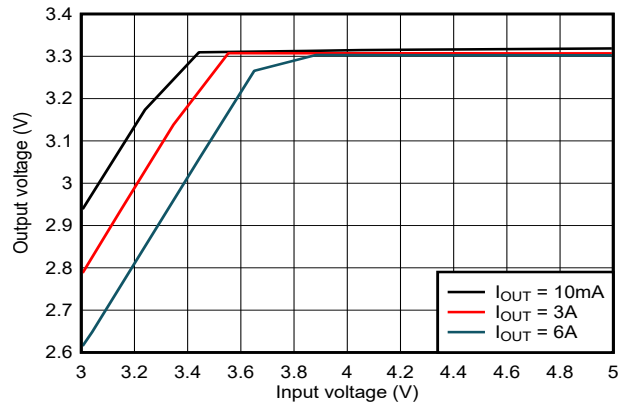
Figure 8-20. Dropout Curve
