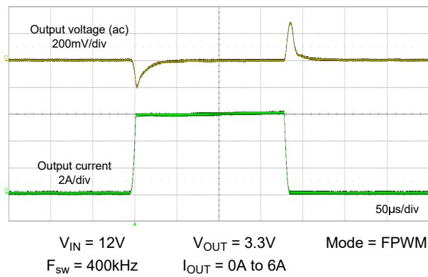
Figure 8-22. Load Transient
