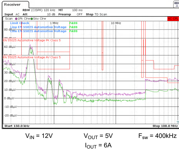
Figure 8-32. Conducted EMI vs CISPR 25 Limits (Pink: Peak Signal, Green: Average Signal)
