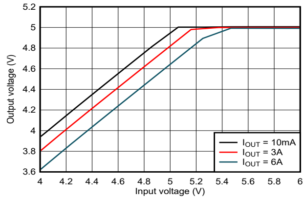
Figure 8-21. Dropout Curve
