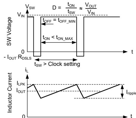
図 7-10. Dropout Waveforms
