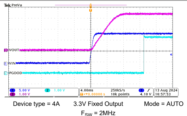
Figure 8-7. Start-Up Operation
