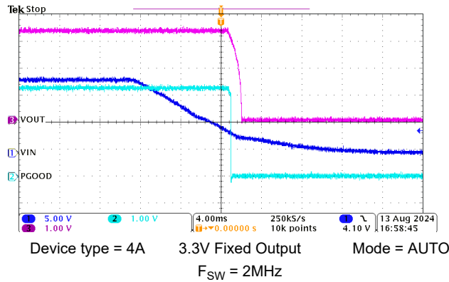
図 8-8. Shutdown Operation
