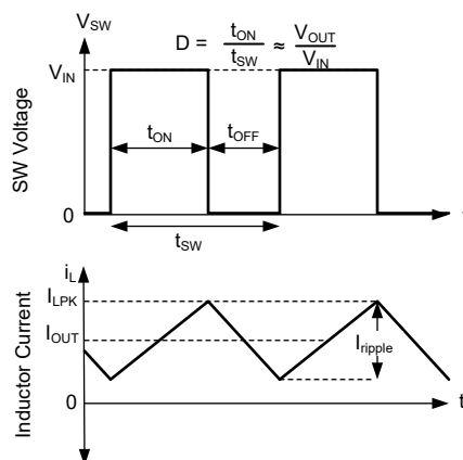
图 7-6. SW Voltage and Inductor Current Waveforms in Continuous Conduction Mode (CCM)
