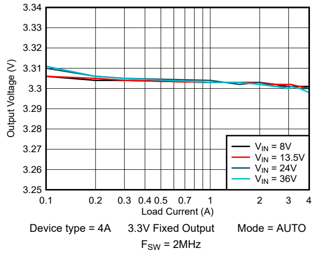
Figure 8-3. Load Regulation
