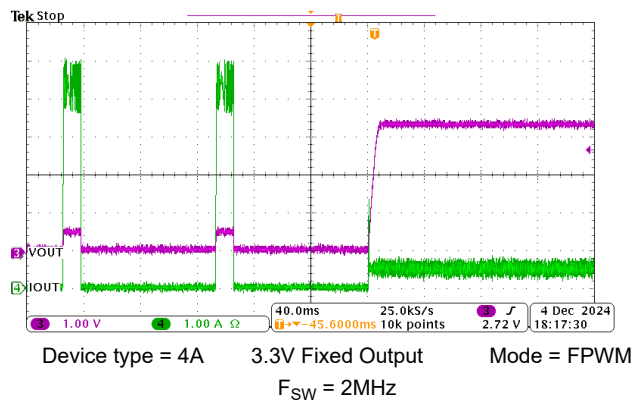
図 8-10. Short-Circuit Recovery
