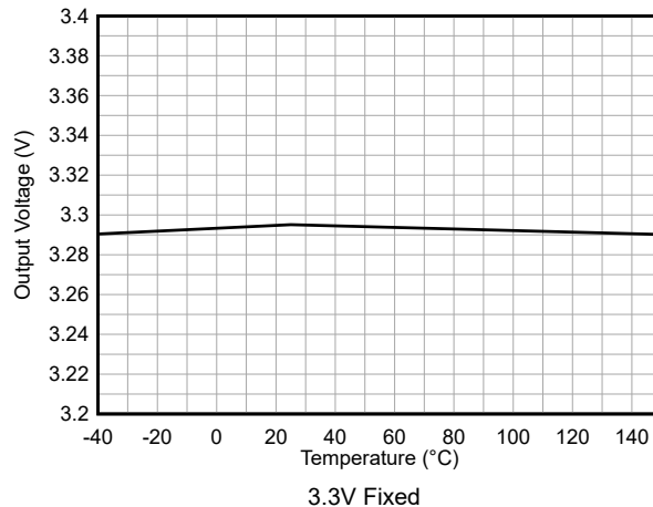
図 6-5. Output Voltage Accuracy
