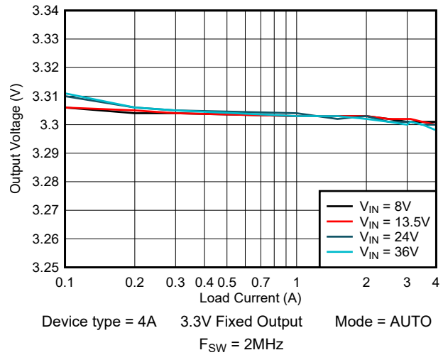
Figure 8-3. Load Regulation
