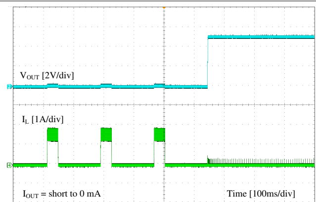
図 8-10. Short Recovery
