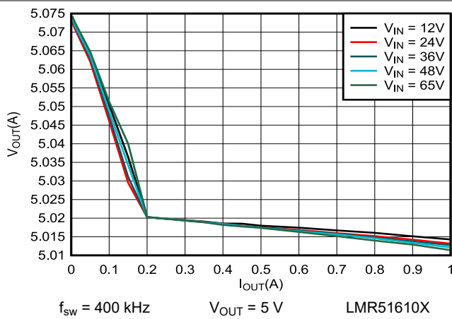
図 6-13. 5-V Load Regulation
