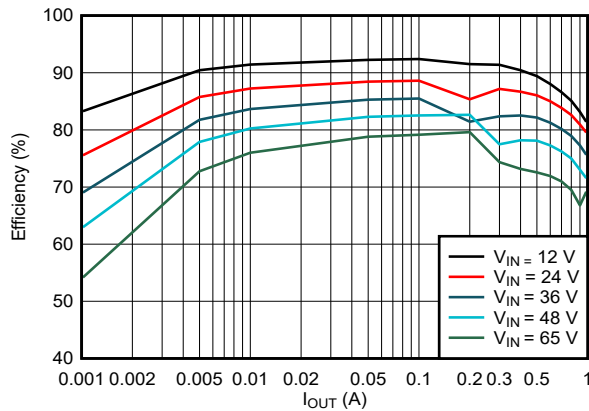
図 6-7. 3.3-V PFM Efficiency Versus Load Current
