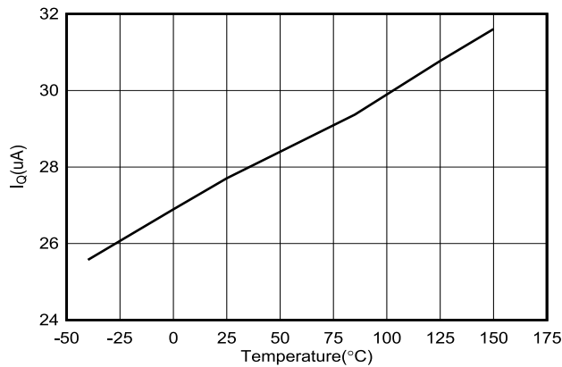
図 6-15. V_{IN} quiescent current Versus Temperature
