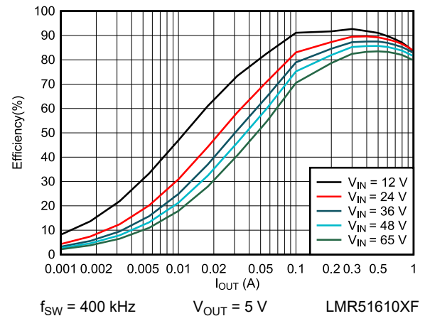
図 6-4. 5-V FPWM Efficiency Versus Load Current
