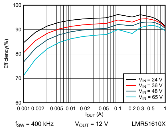
図 6-5. 12-V PFM Efficiency Versus Load Current
