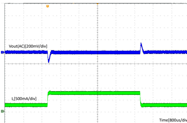
図 8-7. Load Transient (0.25 A – 0.75 A)
