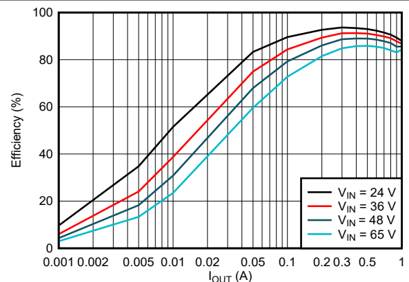
図 6-10. 5-V FPWM Efficiency Versus Load Current
