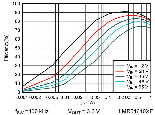
図 6-2. 3.3-V FPWM Efficiency Versus Load Current
