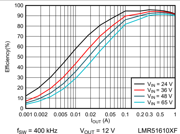
図 6-6. 12-V FPWM Efficiency Versus Load Current
