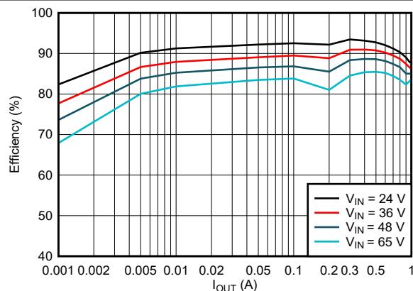
図 6-9. 5-V PFM Efficiency Versus Load Current
