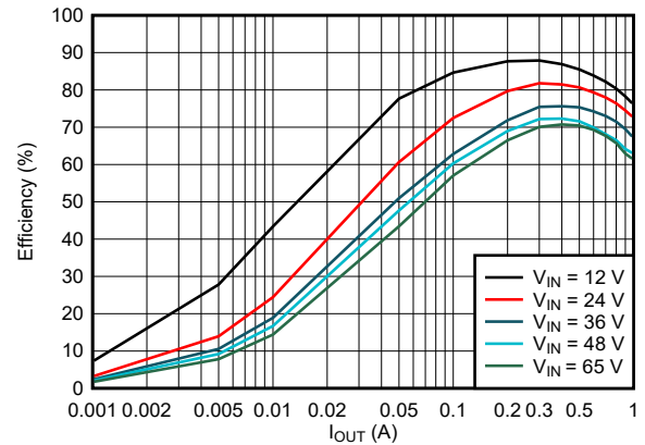
図 6-8. 3.3-V FPWM Efficiency Versus Load Current
