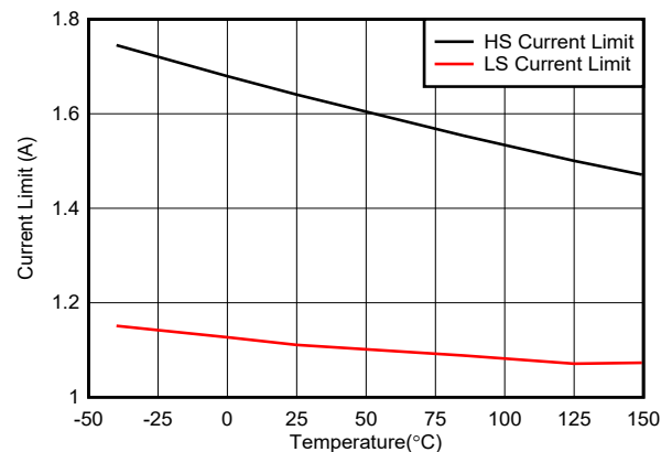
図 6-18. HS and LS Current Limit Versus Temperature
