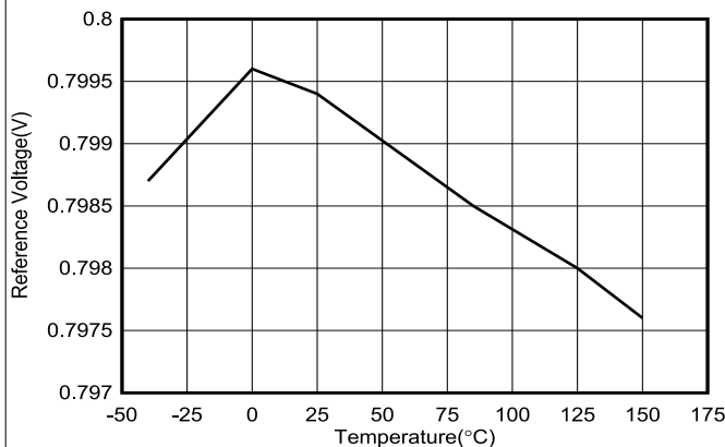
図 6-17. Reference Voltage Versus Temperature
