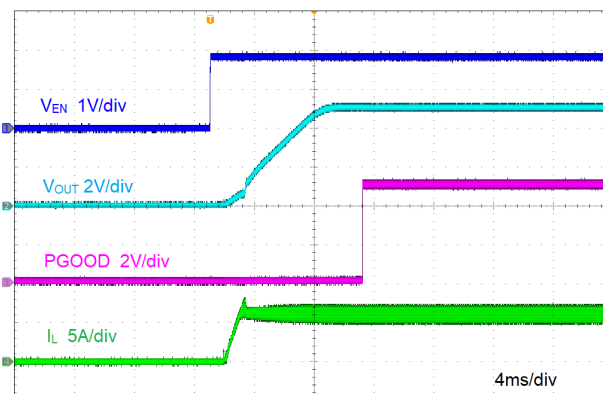
図 8-5. Start-Up by EN
