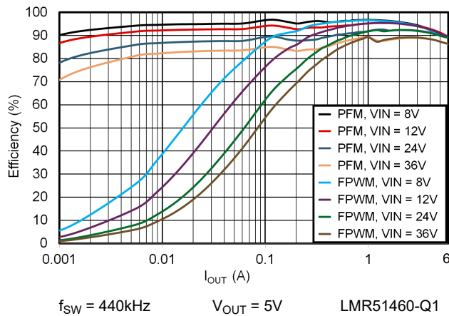
図 6-1. 5V Efficiency versus Load Current
