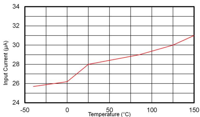
Figure 6-7. Non-Switching Input Supply Current
