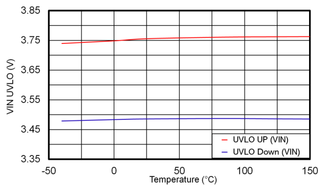
Figure 6-8. V_{IN} UVLO
