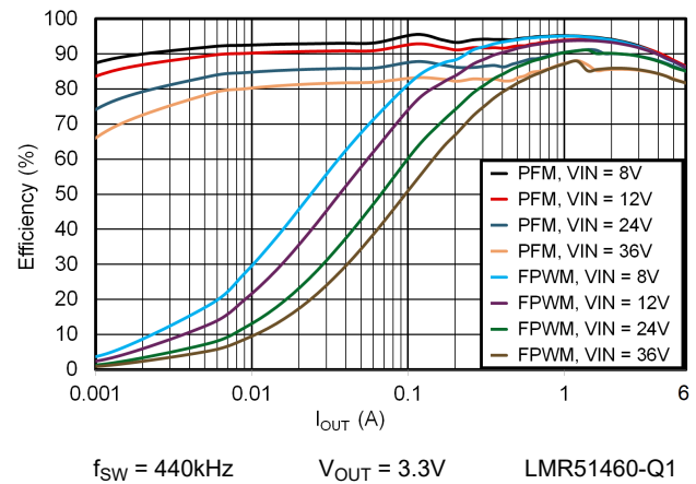
図 6-2. 3.3V Efficiency versus Load Current
