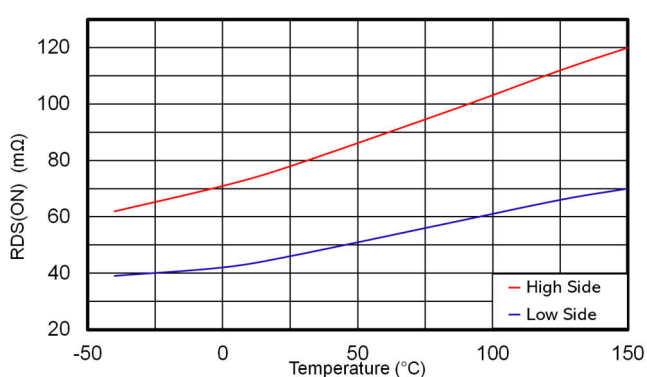
Figure 6-10. High Side and Low Side Switches R_{DS(on)}
