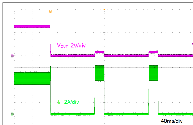
図 8-8. Short Protection
