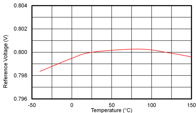
Figure 6-9. Reference Voltage
