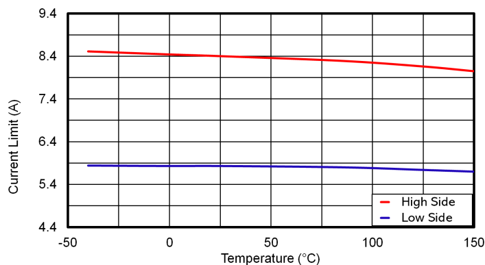
Figure 6-11. LMR51460-Q1 High Side and Low Side Current Limits
