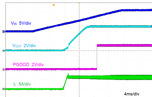
図 8-4. Start-Up by V_{IN}
