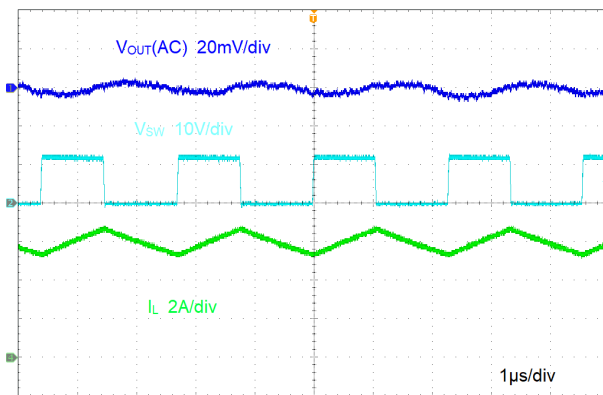
図 8-3. Ripple at Full Load
