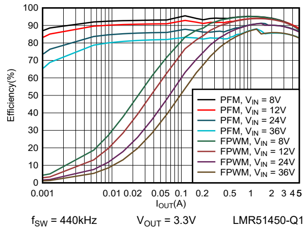
図 6-3. 3.3V Efficiency versus Load Current
