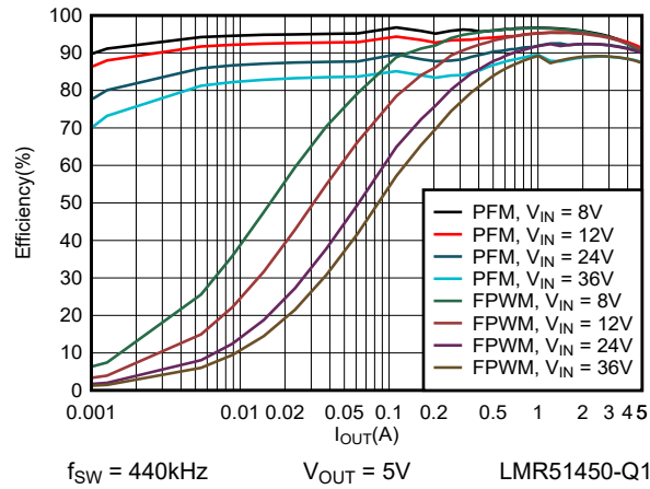
図 6-1. 5V Efficiency versus Load Current
