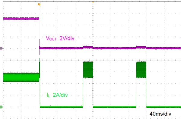
図 8-8. Short Protection
