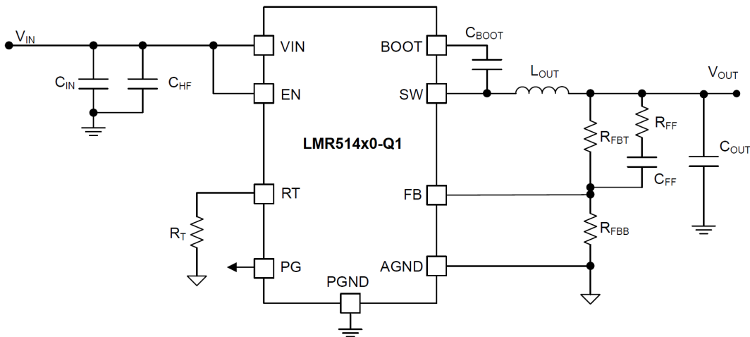
図 8-1. Application Circuit
