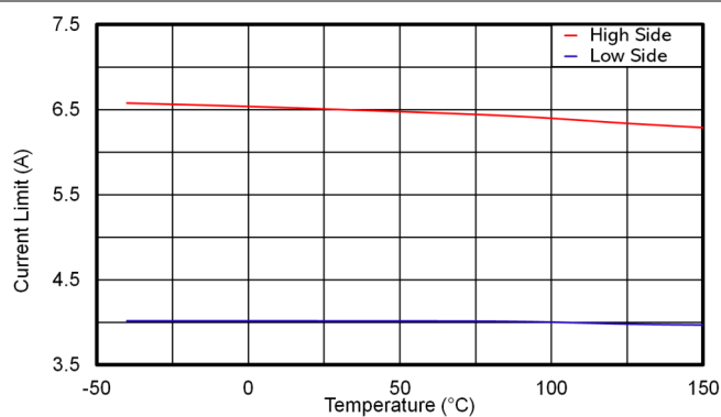
FIG 6-14. LMR51440-Q1 High Side and Low Side Current Limits
