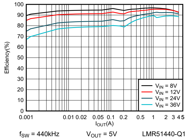
図 6-2. 5V Efficiency versus Load Current
