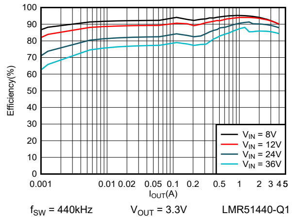
図 6-4. 3.3V Efficiency versus Load Current
