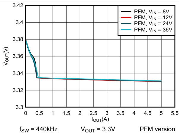
図 6-5. 3.3V Load Regulation
