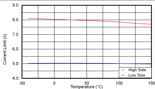
FIG 6-13. LMR51450-Q1 High Side and Low Side Current Limits
