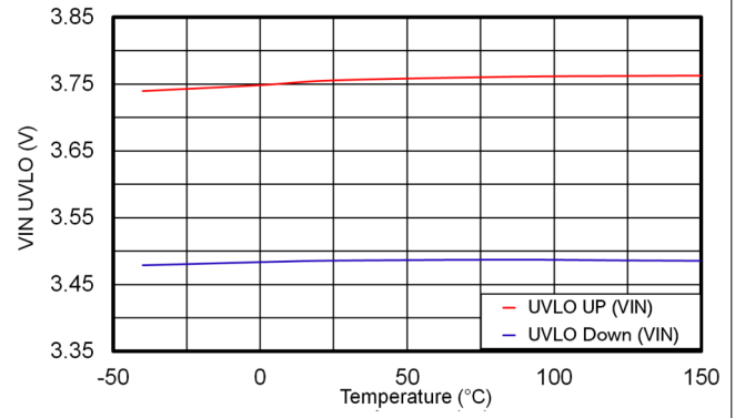
Figure 6-10. V_{IN} UVLO
