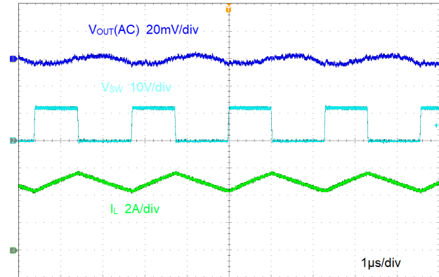
図 8-3. Ripple at Full Load
