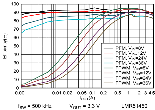
7-3. 3.3-V Efficiency versus Load Current
