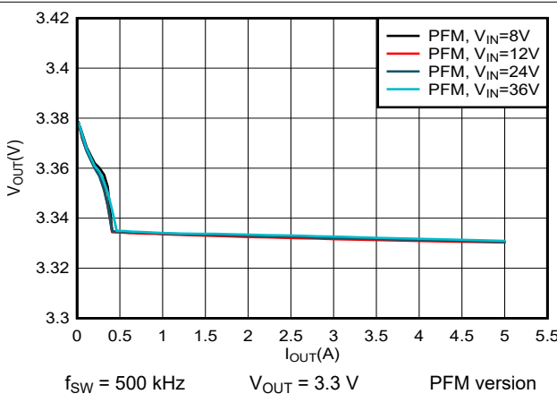
7-5. 3.3-V Load Regulation
