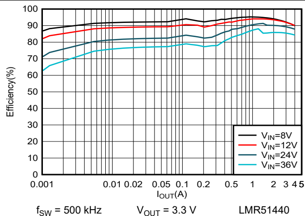
7-4. 3.3-V Efficiency versus Load Current
