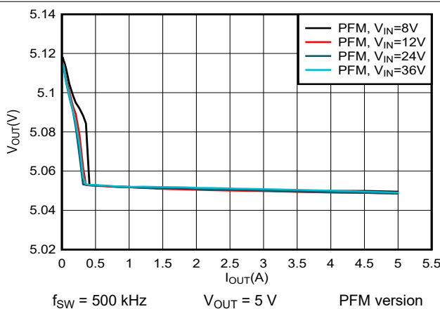
7-6. 5-V Load Regulation
