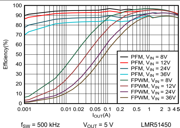
7-1. 5-V Efficiency versus Load Current
