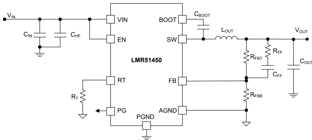
图 9-1. Application Circuit
