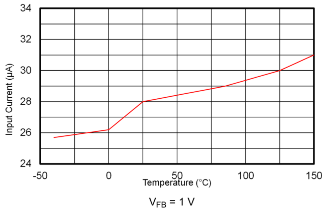
7-9. Non-Switching Input Supply Current
