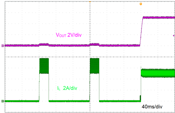
Figure 9-9. Short Recovery
