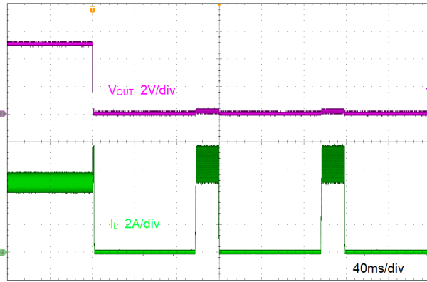
Figure 9-8. Short Protection
