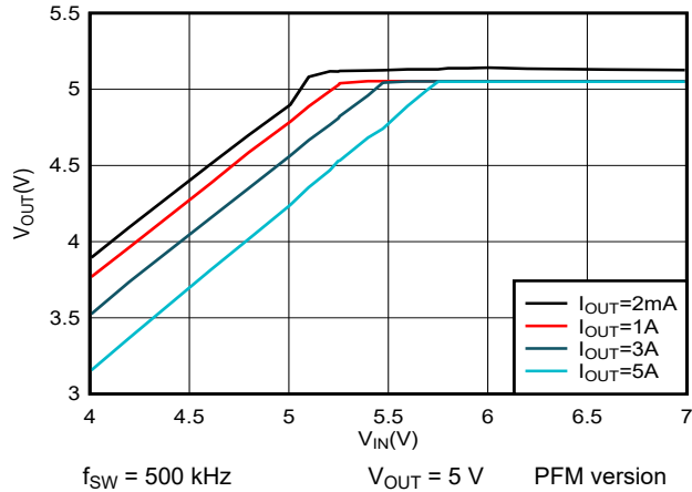
7-7. 5-V Dropout
