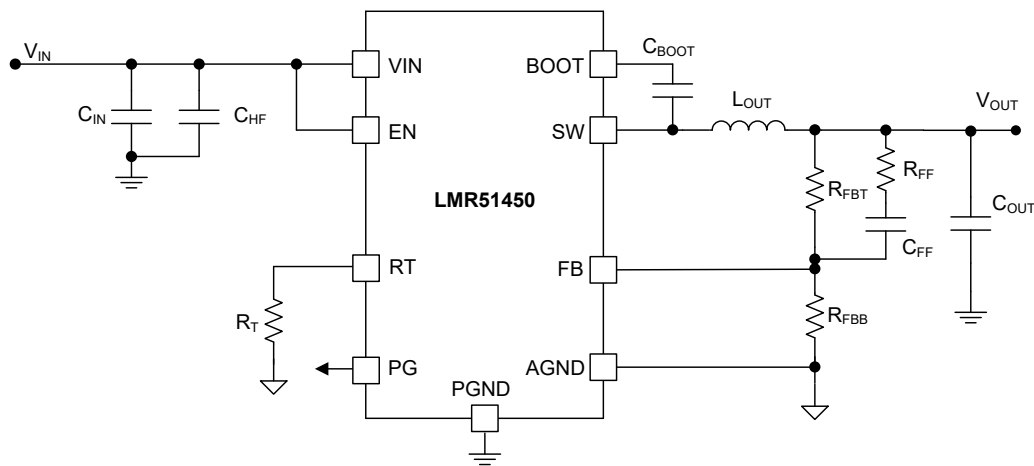
图 9-1. Application Circuit
