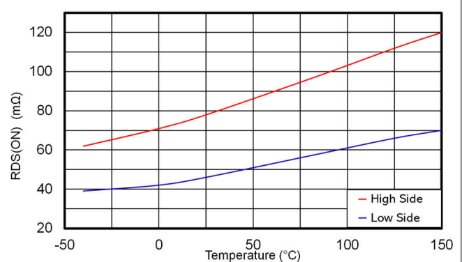
7-12. High Side and Low Side Switches R_{DS\_ON}
