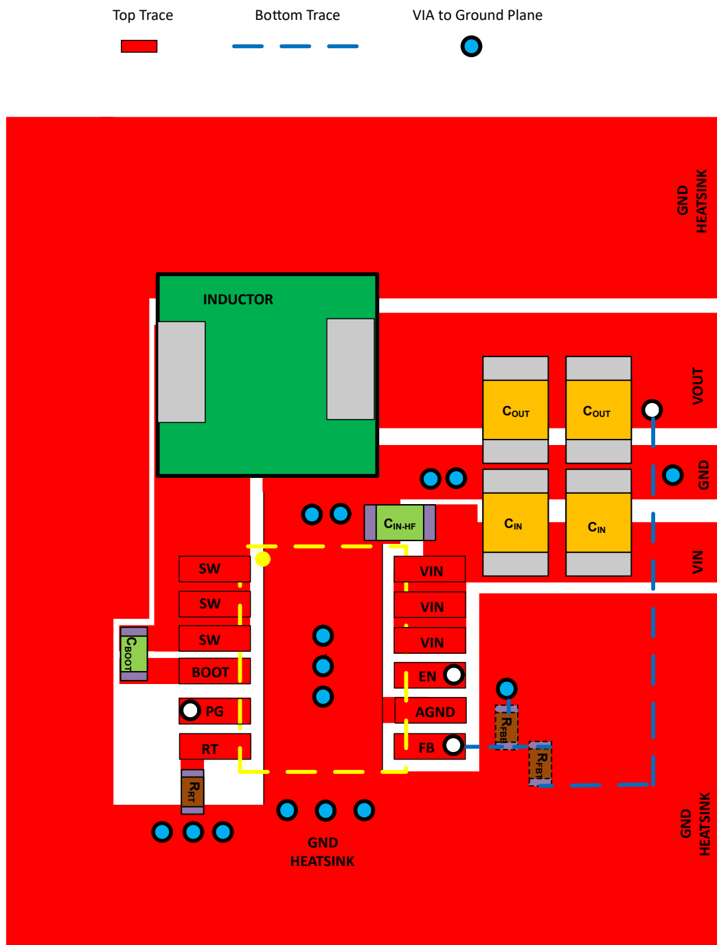
9-10. Layout
