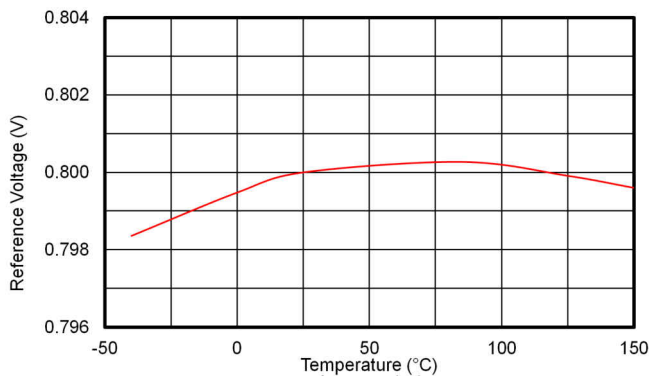
7-11. Reference Voltage
