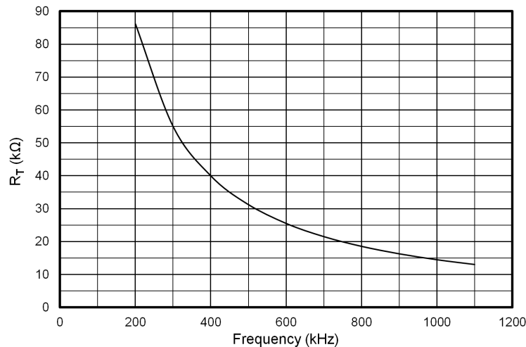
図 8-4. R_T Versus Frequency Curve
