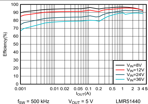
7-2. 5-V Efficiency versus Load Current
