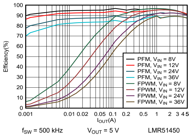
7-1. 5-V Efficiency versus Load Current
