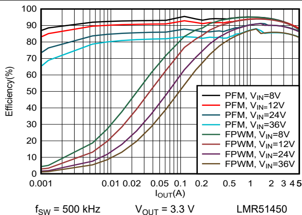
7-3. 3.3-V Efficiency versus Load Current
