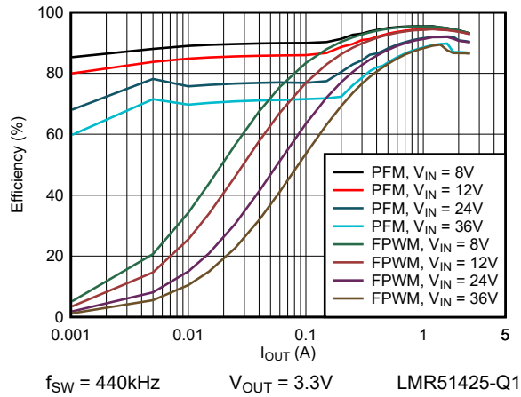
図 6-7. 3.3V Efficiency versus Load Current
