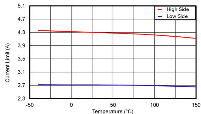
図 6-18. LMR51425-Q1 High Side and Low Side Current Limits
