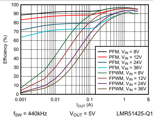
図 6-5. 5V Efficiency versus Load Current
