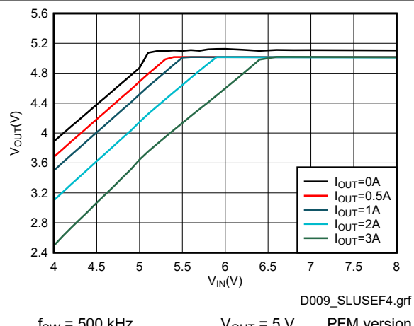
7-6. 5-V Dropout
