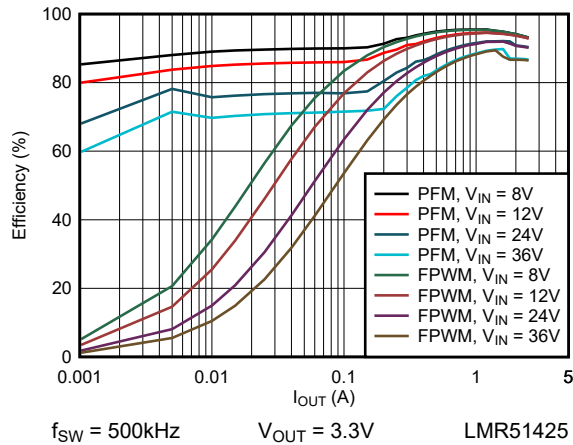
図 6-7. 3.3V Efficiency versus Load Current
