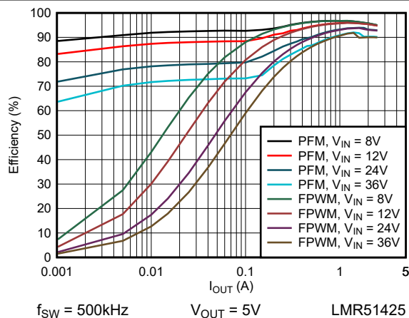
図 6-5. 5V Efficiency versus Load Current
