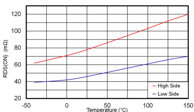
図 6-16. High Side and Low Side Switches R_{DS(on)}
