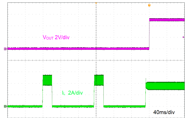
8-9. Short Recovery
