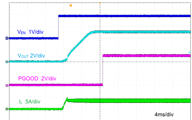
図 8-5. Start-Up by EN
