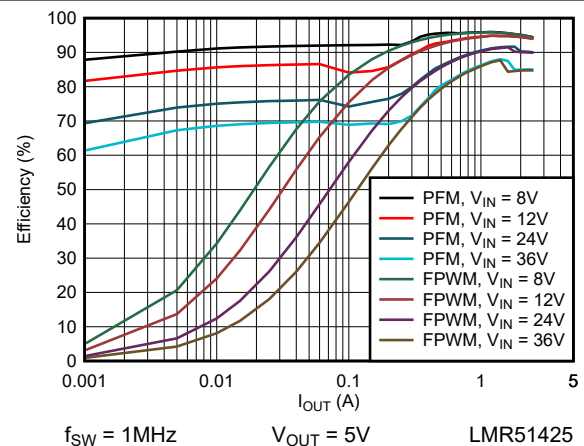
図 6-6. 5V Efficiency versus Load Current
