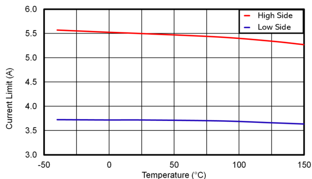
図 6-17. LMR51435 High Side and Low Side Current Limits
