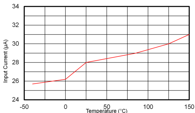
図 6-13. Non-Switching Input Supply Current
