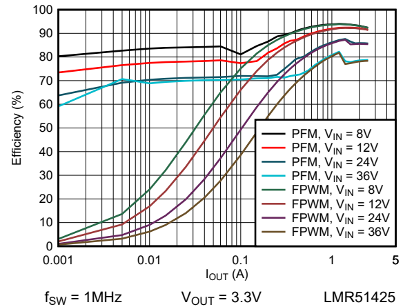
図 6-8. 3.3V Efficiency versus Load Current
