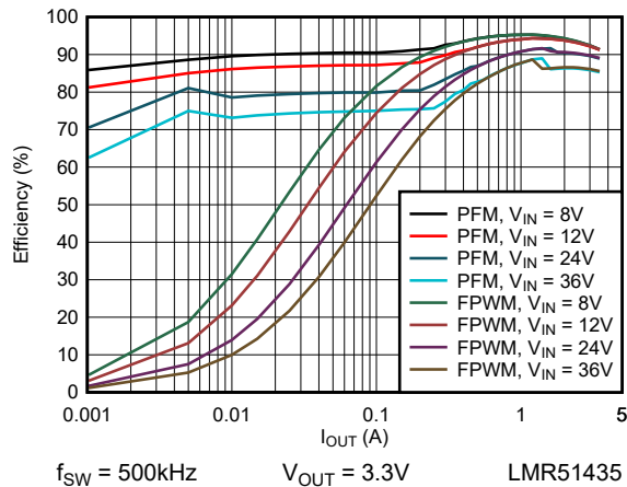
図 6-3. 3.3V Efficiency versus Load Current
