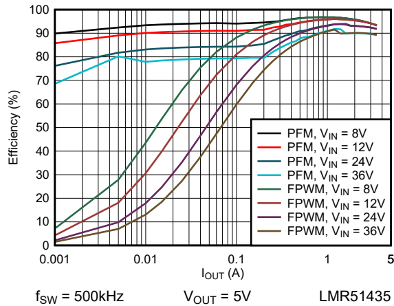
図 6-1. 5V Efficiency versus Load Current
