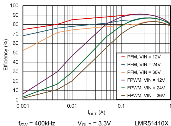
図 6-1. 3.3V Efficiency Versus Load Current
