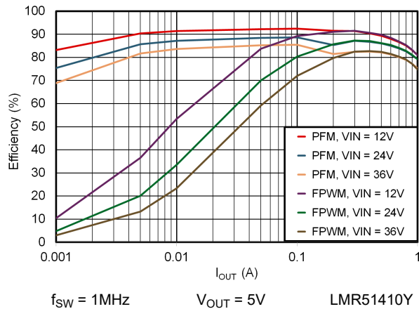
図 6-5. 5V Efficiency Versus Load Current
