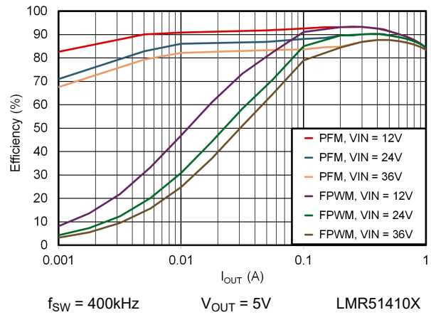
図 6-2. 5V Efficiency Versus Load Current
