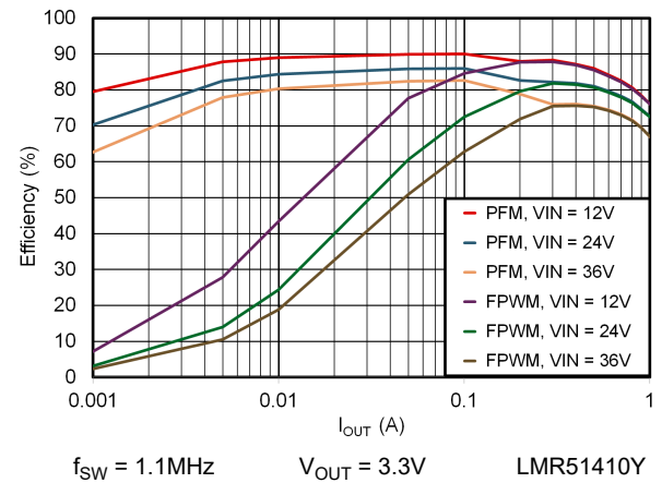
図 6-4. 3.3V Efficiency Versus Load Current
