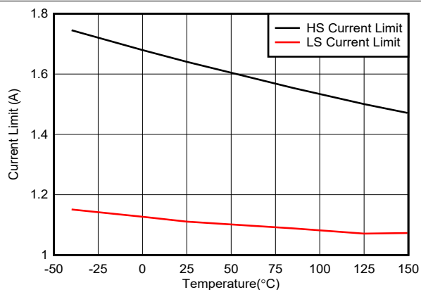
図 6-12. HS and LS Current Limit Versus Temperature
