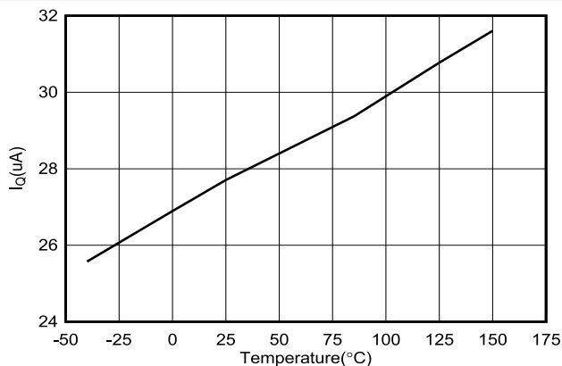
図 6-9. V_{IN} Quiescent Current Versus Temperature
