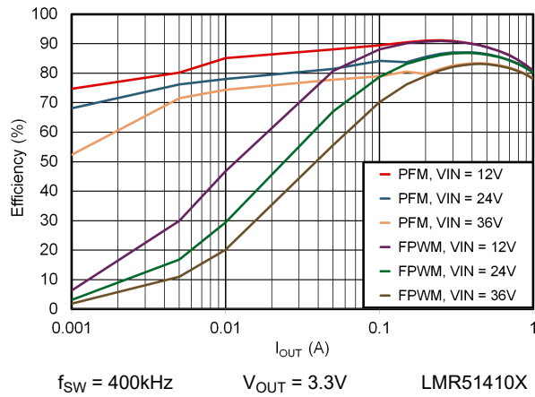
図 6-1. 3.3V Efficiency Versus Load Current
