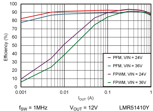
図 6-6. 12V Efficiency Versus Load Current
