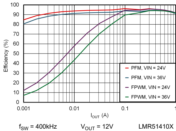
図 6-3. 12V Efficiency Versus Load Current
