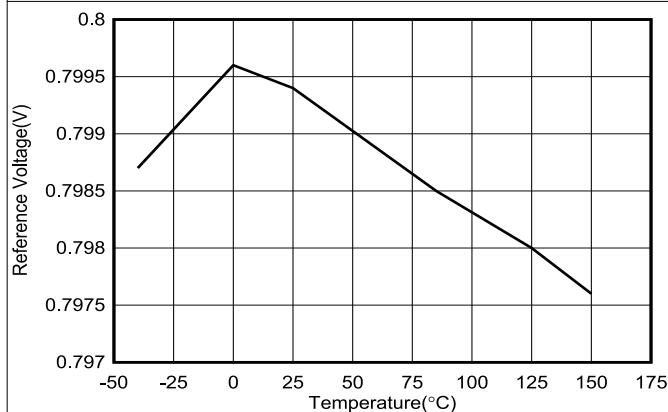
図 6-11. Reference Voltage Versus Temperature
