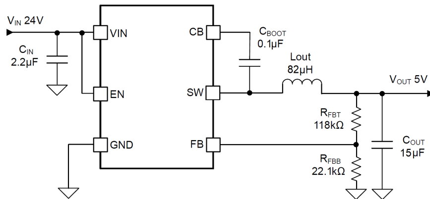
図 8-1. Application Circuit
