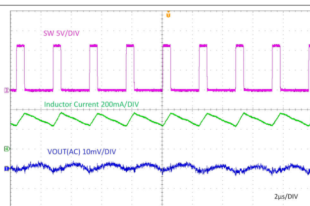
図 8-4. Ripple at Full Load
