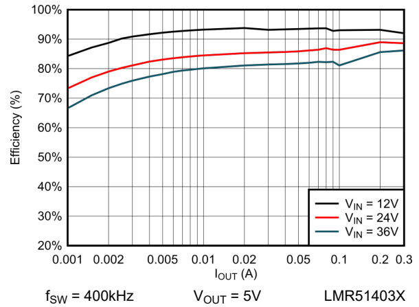
図 6-2. 5V Efficiency vs Load Current
