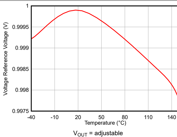
Figure 6-4. Feedback Voltage Accuracy Versus Temperature
