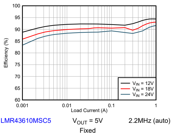
図 8-5. Efficiency
