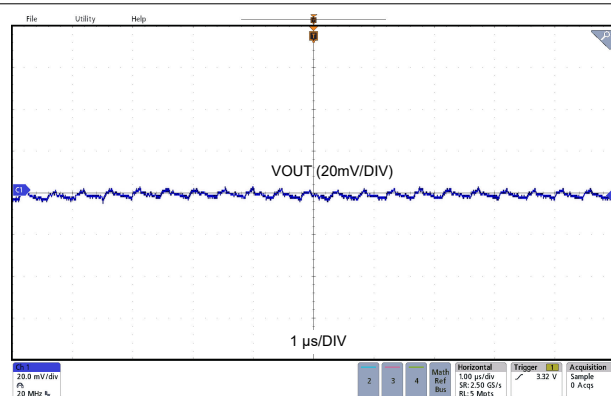
LMR43620MSC3 V_{OUT} = 3.3V 2A load Fixed
