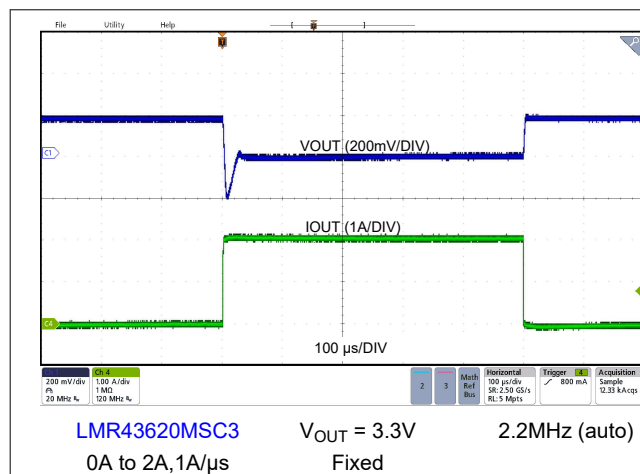
8-15. Load Transient
