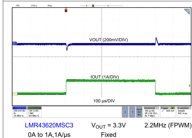
8-17. Load Transient
