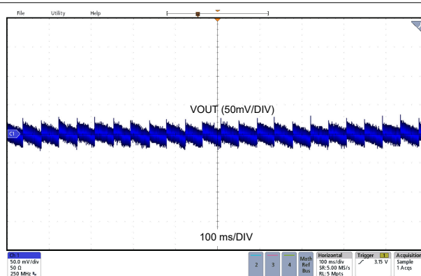
LMR43620MSC3 V_{OUT} = 3.3V No load Fixed
