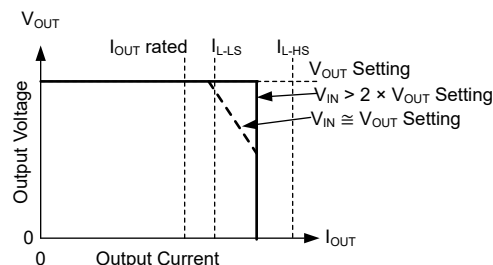
☒ 7-14. Output Voltage Versus Output Current
