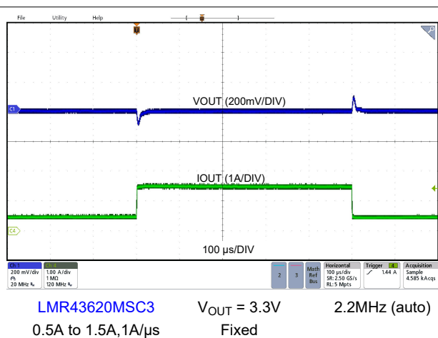
8-16. Load Transient
