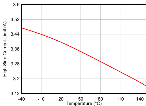
Figure 6-5. High Side MOSFET Current Limit Versus Temperature
