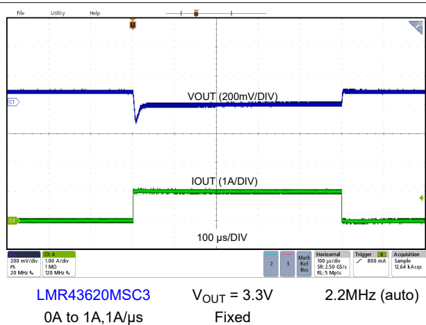
8-18. Load Transient
