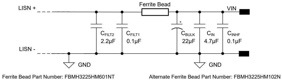
図 8-29. Typical Input EMI Filter
