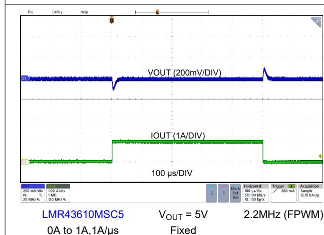
8-19. Load Transient
