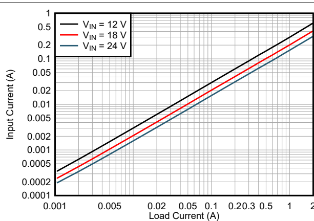
LMR43620MSC3 V_{OUT} = 3.3V 2.2MHz (auto) Fixed
