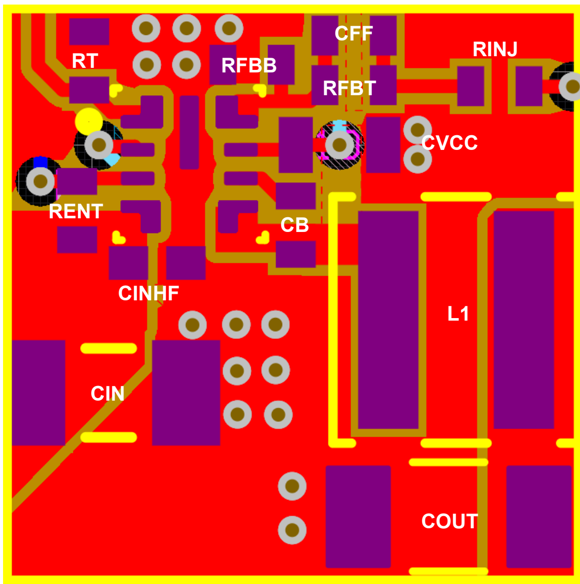
Figure 8-32. Example Layout
