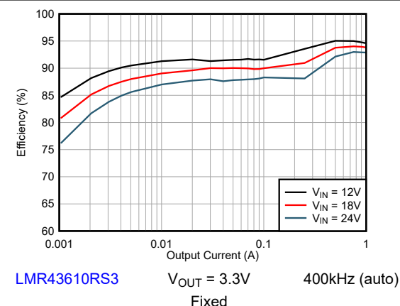
図 8-8. Efficiency
