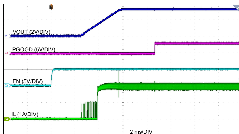
図 7-3. Enable Start-Up V_{IN} = 12V , V_{OUT} = 3.3V , I_{OUT} = 2A
