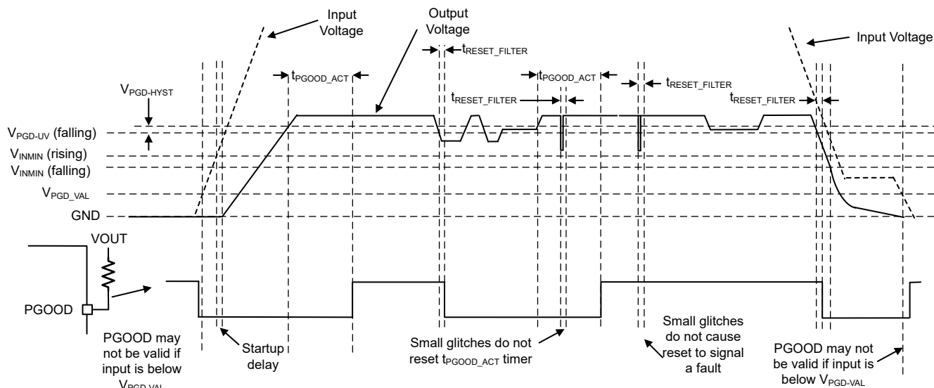
8-8. Power-Good Operation (OV Events Not Included)
