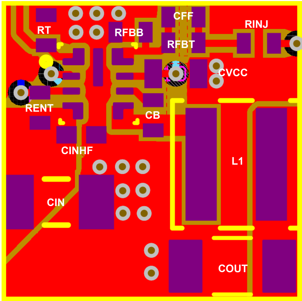
Figure 9-23. Example Layout
