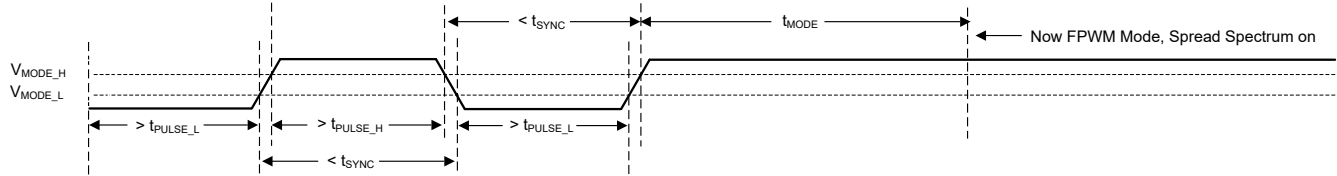
図 8-6. Transition from SYNC Mode to FPWM Mode
