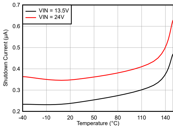
FIG 7-1. Shutdown Current Versus Temperature
