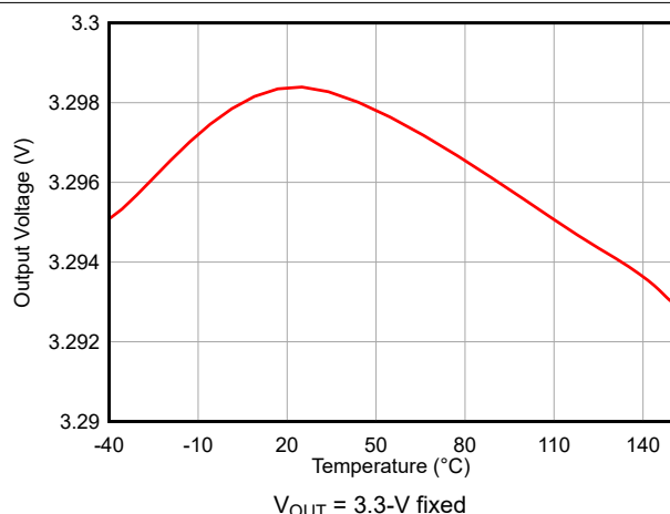
FIG 7-3. Output Voltage Accuracy Versus Temperature
