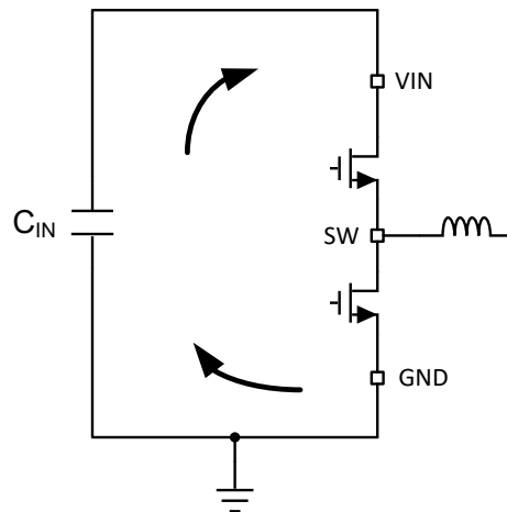
図 9-22. Current Loops with Fast Edges
