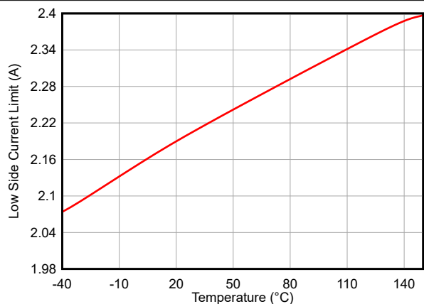
FIG 7-6. Low Side MOSFET Current Limit Versus Temperature
