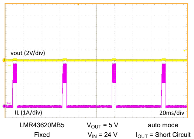
图 9-12. Short-Circuit Performance
