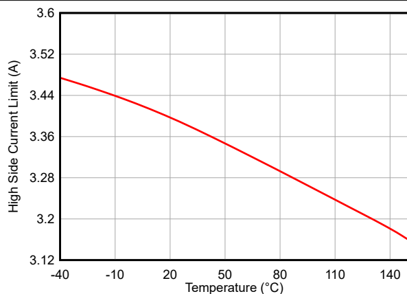
FIG 7-5. High Side MOSFET Current Limit Versus Temperature
