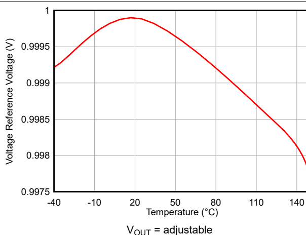
FIG 7-4. Feedback Voltage Accuracy Versus Temperature
