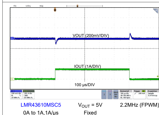
8-19. Load Transient
