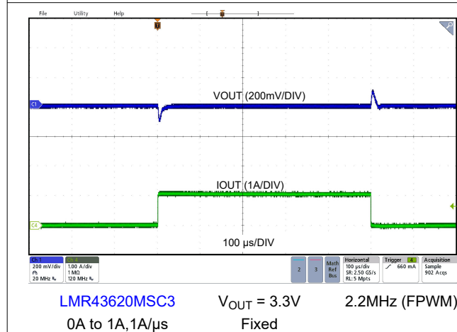
8-17. Load Transient
