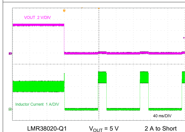
8-7. Short Circuit Applied
