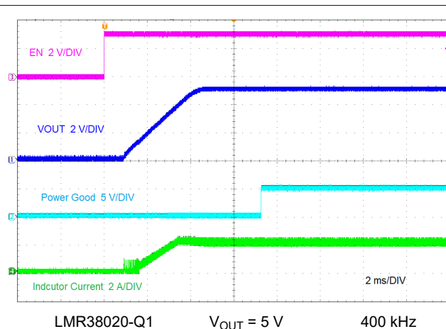
8-4. Start-Up by EN
