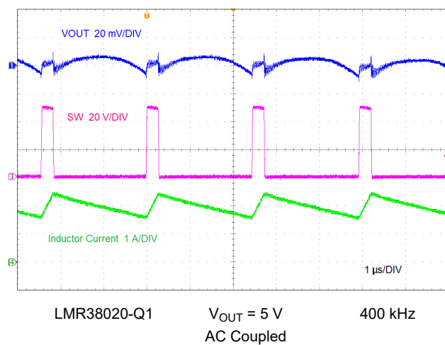
8-6. Full Load Switching
