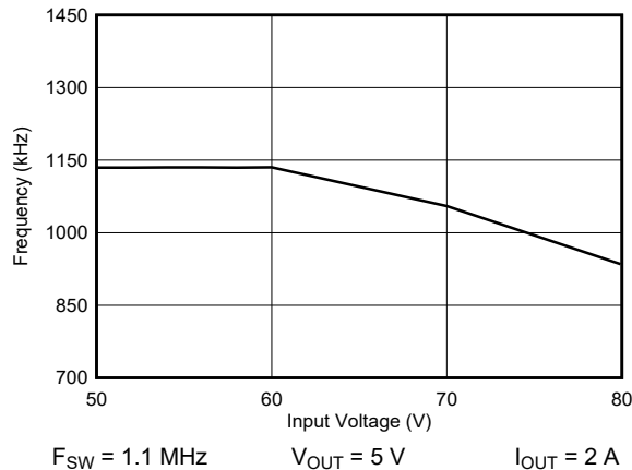
7-8. Typical Frequency Foldback at T_{ON\_MIN}
