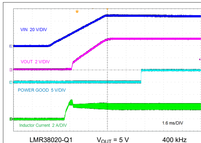
8-3. Start-Up by VIN
