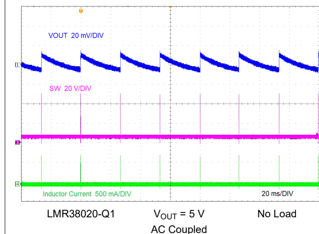
8-5. PFM Switching
