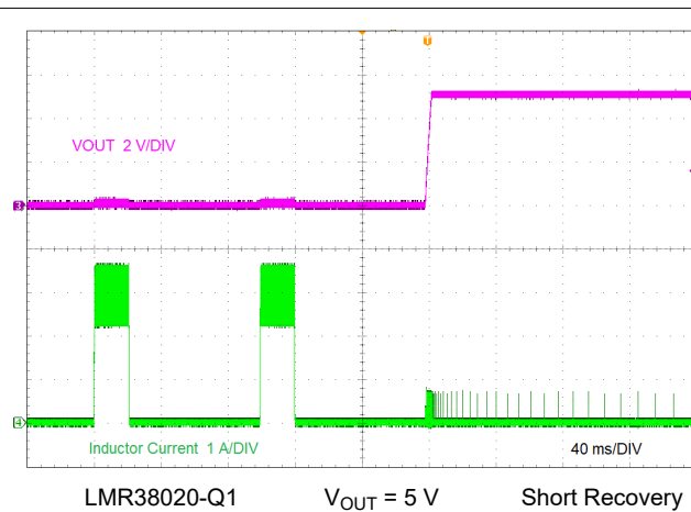
8-8. Short-Circuit Recovery
