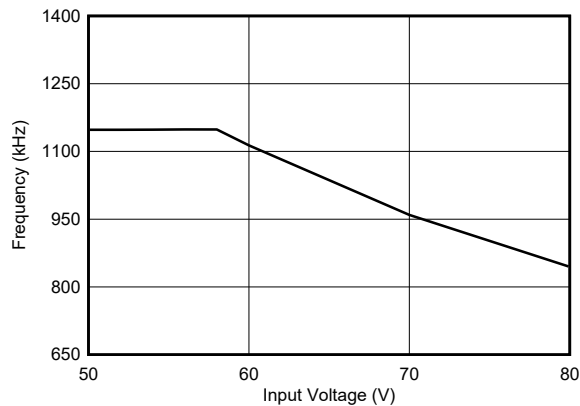
F_{SW} = 1.1 \text{ MHz} V_{OUT} = 5 \text{ V} I_{OUT} = 1 \text{ A} Figure 7-8. Typical Frequency Foldback at T_{ON\_MIN}
