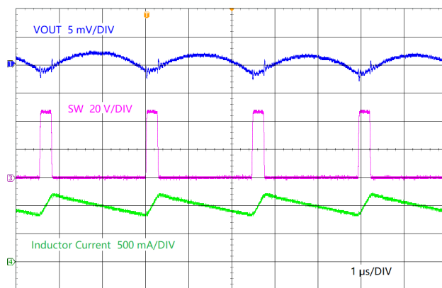
LMR38010-Q1 V_{OUT} = 5\text{ V} 400 kHz AC Coupled
