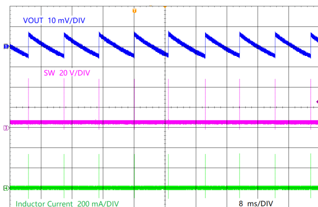
LMR38010-Q1 V_{OUT} = 5\text{ V} No Load AC Coupled
