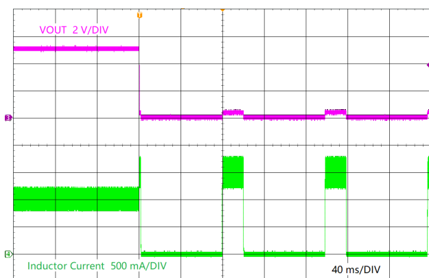
LMR38010-Q1 V_{OUT} = 5\text{ V} 1 A to Short
