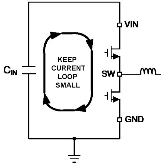
8-15. Current Loops with Fast Edges
