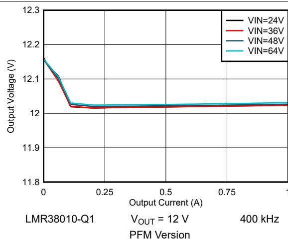
8-14. 12-V Load Regulation
