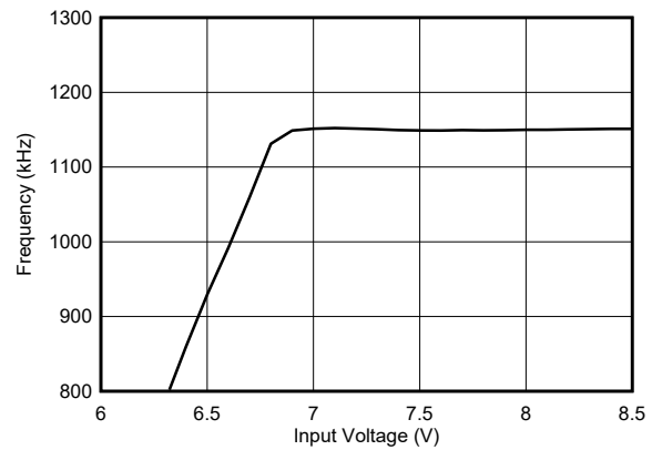
F_{SW} = 1.1 \text{ MHz} V_{OUT} = 5 \text{ V} I_{OUT} = 1 \text{ A} Figure 7-9. Typical Frequency Foldback at T_{OFF\_MIN}
