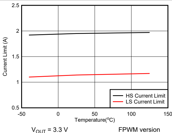
图 6-5. High-Side and Low-Side Current Limit vs Temperature
