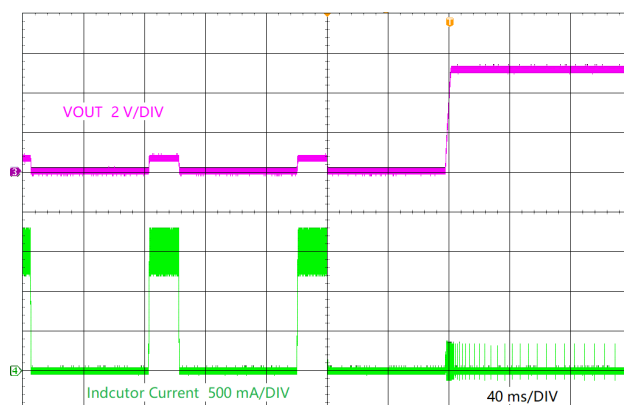
LMR38010-Q1 V_{OUT} = 5\text{ V} Short Recovery
