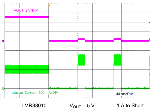
図 9-7. Short Circuit Applied
