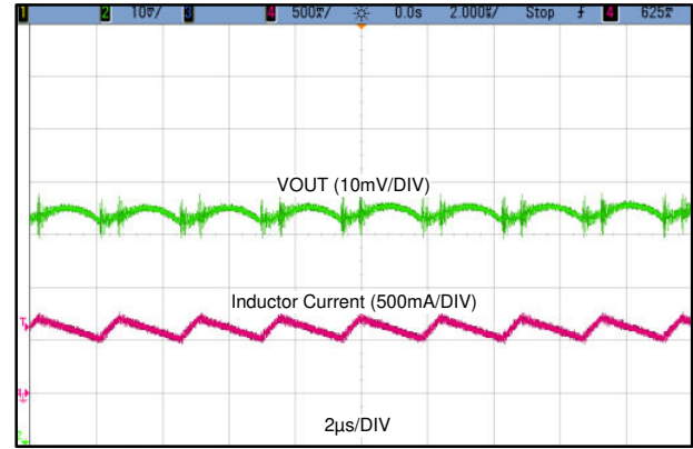
9-17. Output Ripple
