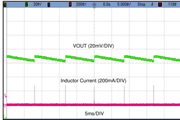
9-16. Output Ripple
