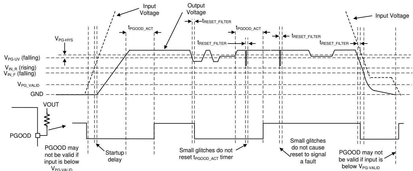
図 8-8. Power-Good Operation (OV Events Not Included)
