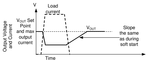
FIG 8-11. Recovery from Dropout
