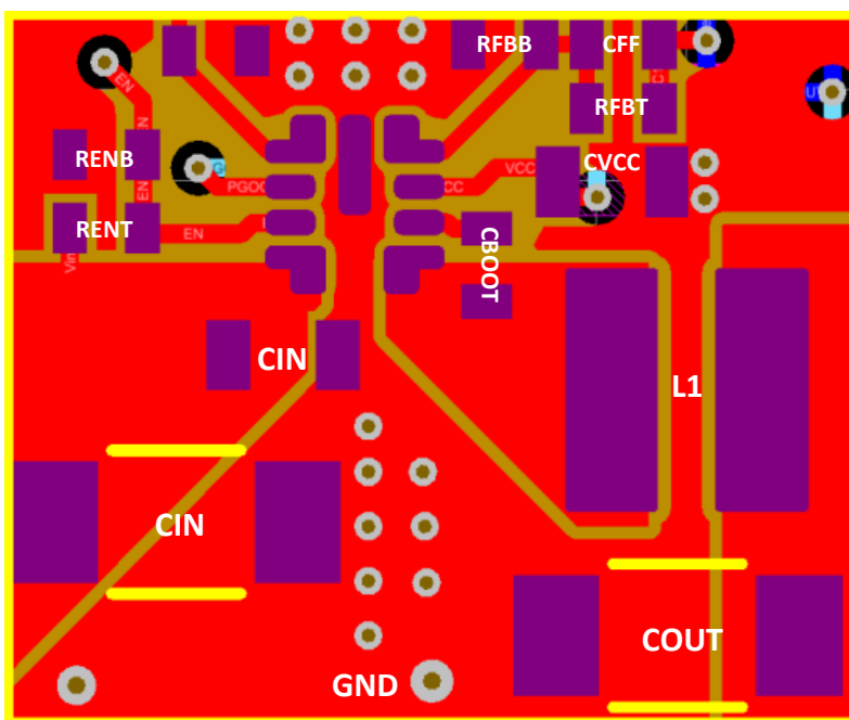
11-2. Example Layout
