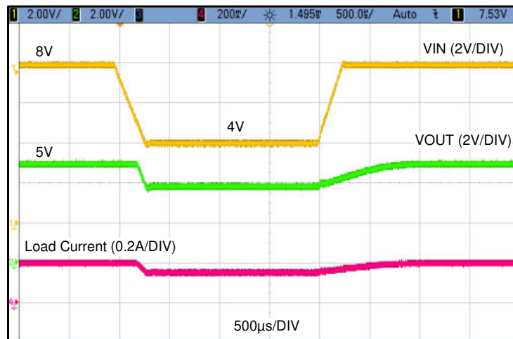
FIG 8-12. Typical Output Recovery from Dropout from 8 V to 4 V
