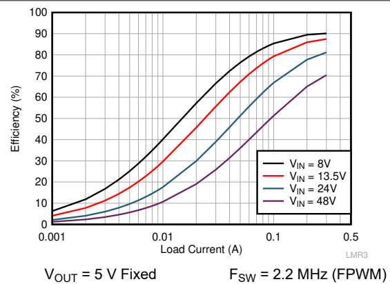
7-2. Efficiency 5-V Output, FPWM
