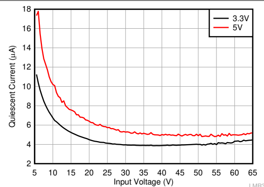
7-4. Typical Input Supply Current at No Load for Fixed 3.3-V and 5-V Output
