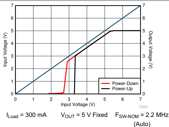
7-5. Dropout at Power-Up and Power-Down
