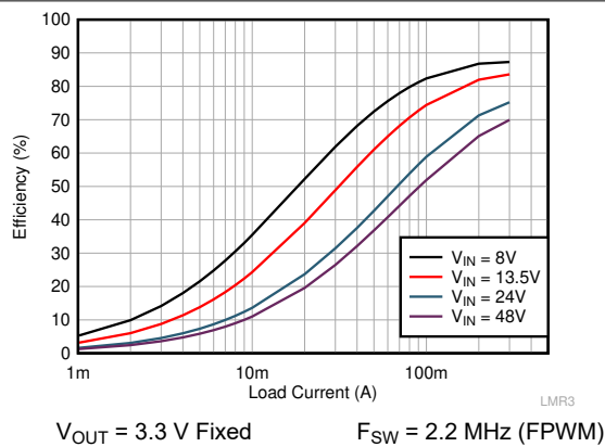
7-1. Efficiency 3.3-V Output, FPWM
