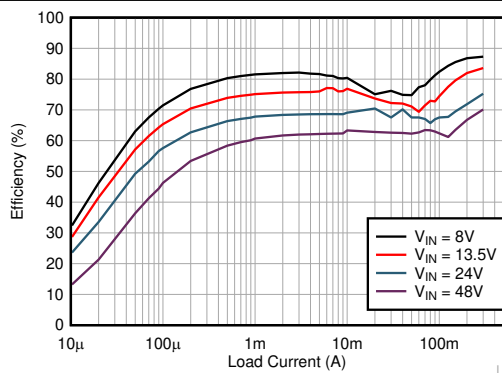
LMR36503MSC3 V_{OUT} = 3.3 V Fixed 2.2 MHz (AUTO)
