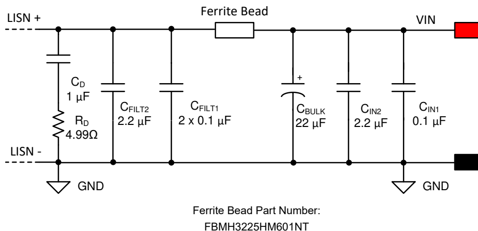
9-24. Typical Input EMI Filter for 2.2 MHz
