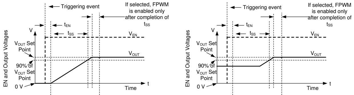
FIG 8-10. Soft Start With and Without Pre-bias Voltage
