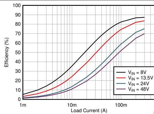
LMR36503MSC3 V_{OUT} = 3.3 V Fixed 2.2 MHz (FPWM)
