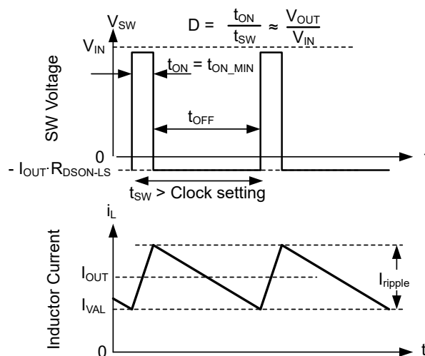
8-14. Valley Current Mode Operation
