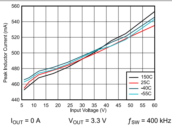
8-6. I_{PEAK-MIN}
