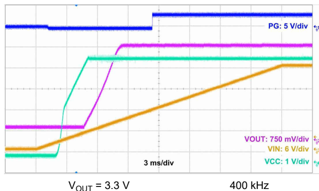
10-15. Start-Up Waveform
