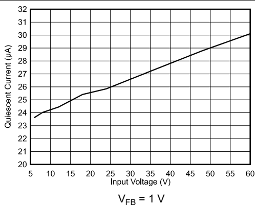
8-1. Non-Switching Input Supply Current
