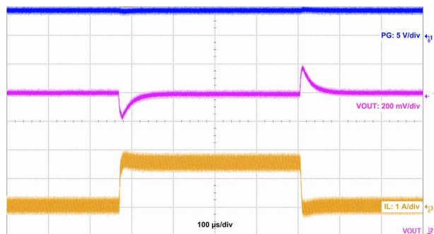
✎ 10-35. Load Transient
