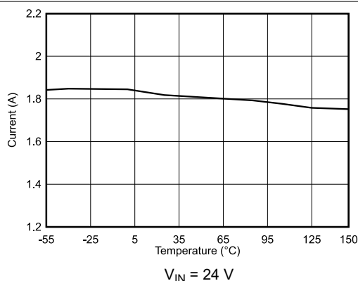
8-4. Low Side Current Limit
