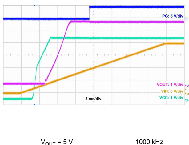
FIG 10-33. Start-Up Waveform
