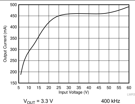
10-13. Mode Change Thresholds
