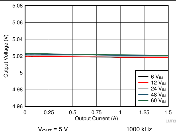
FIG 10-29. Load Regulation
