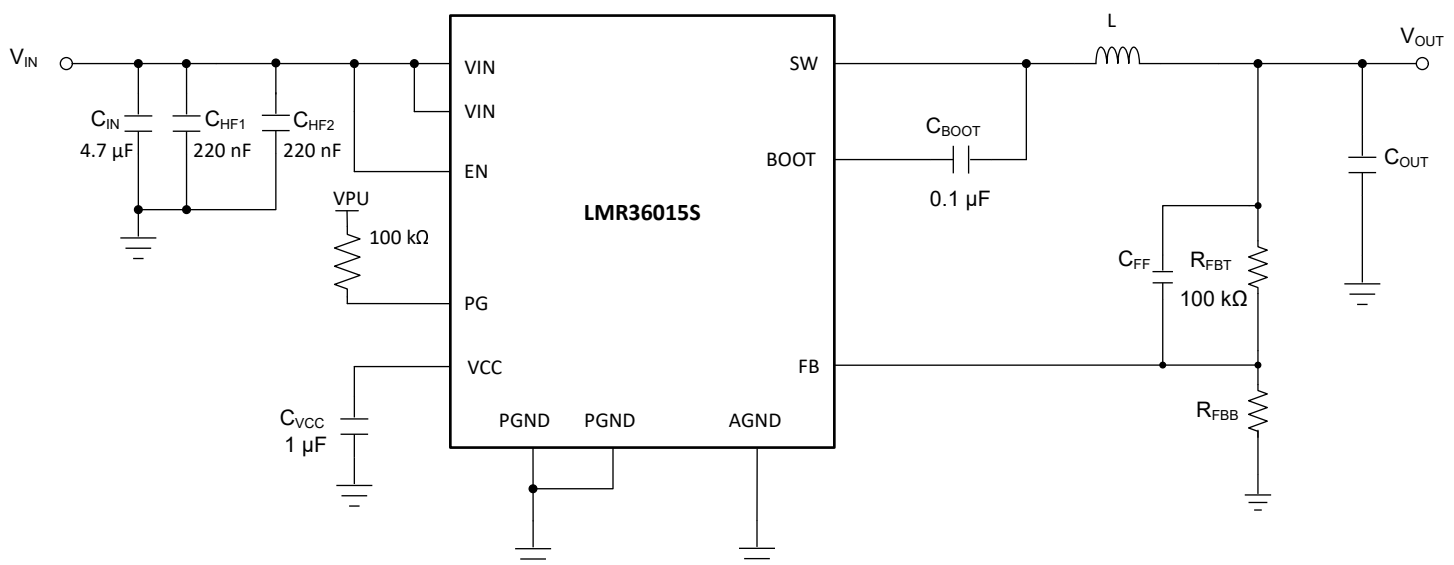
図 10-1. Example Applications Circuit
