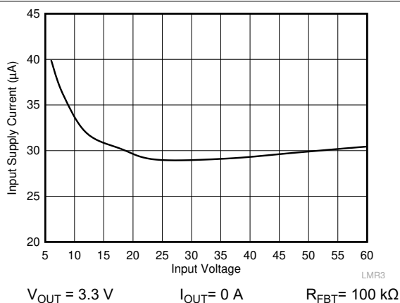
FIG 10-12. Input Supply Current
