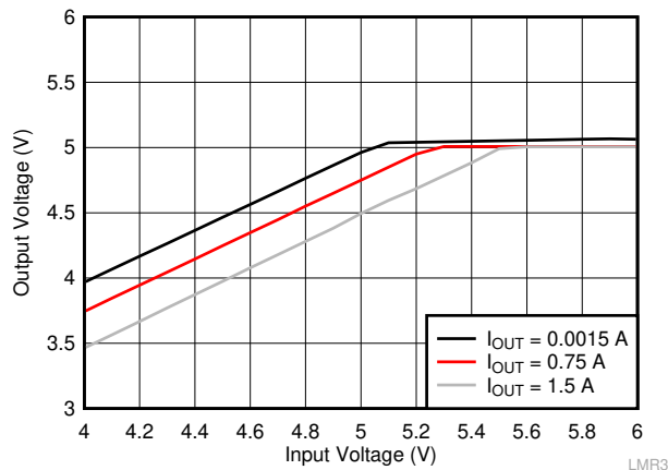
Figure 9-9. Overall Dropout Characteristic V_{OUT} = 5\text{ V}
