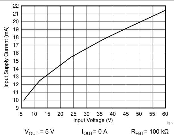
10-32. Input Supply Current
