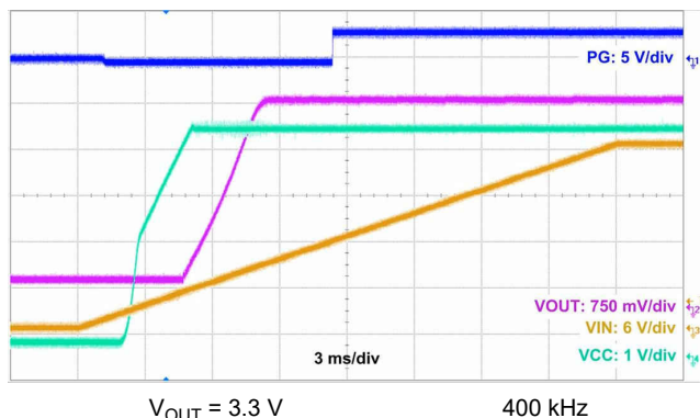
FIG 10-15. Start-Up Waveform
