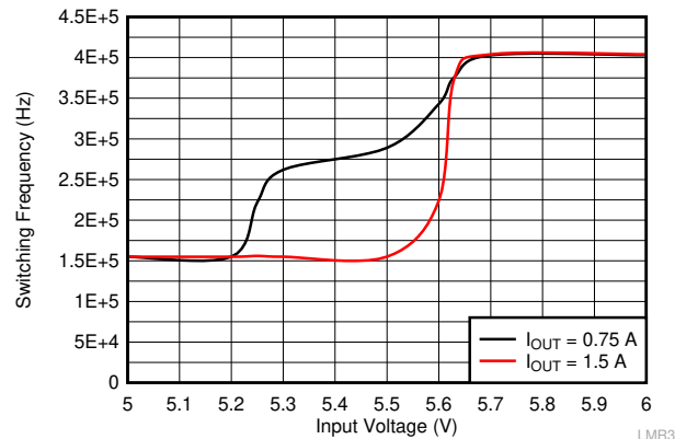
Figure 9-10. Frequency Dropout Characteristics f_{sw} = 400\text{ kHz}
