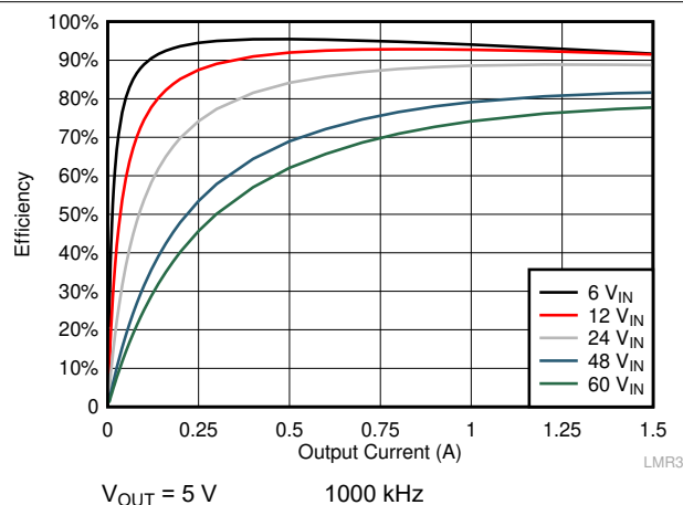
10-28. Efficiency
