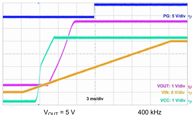
FIG 10-14. Start-Up Waveform
