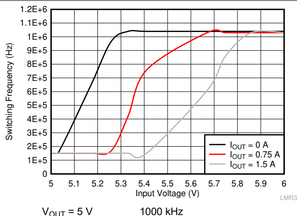
10-31. Frequency Dropout Characteristic
