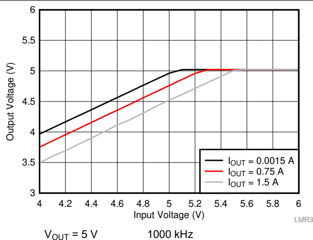
10-30. Overall Dropout Characteristic
