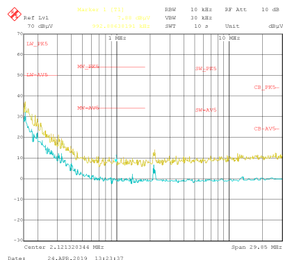
9-17. Conducted EMI vs. CISPR25 Limits (Yellow: Peak Signal, Blue: Average Signal)
