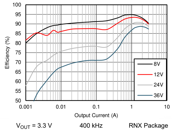
Figure 8-6. Efficiency
