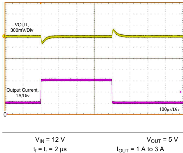
8-16. Load Transient
