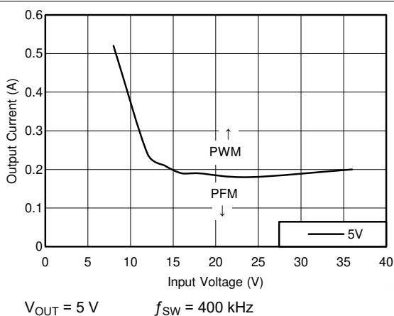
8-13. Mode Change Thresholds
