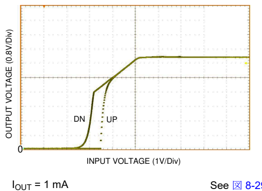
Figure 6-5. UVLO Thresholds
