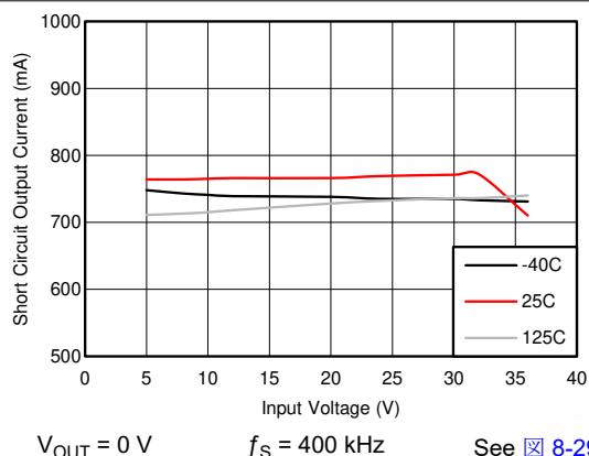
6-3. Short-Circuit Output Current
