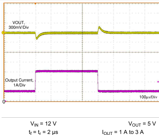
8-16. Load Transient
