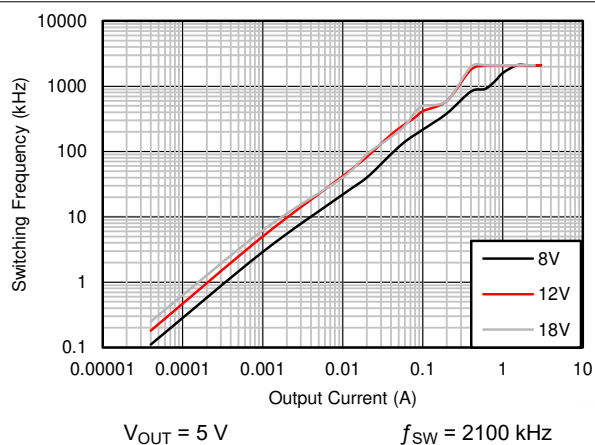
8-14. Switching Frequency versus Output Current
