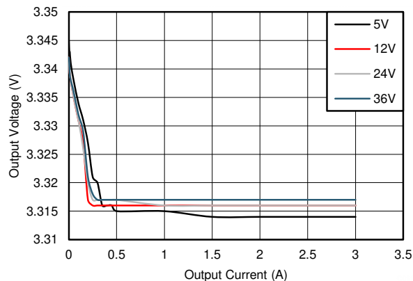
8-17. Line and Load Regulation
