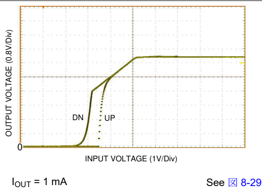
図 6-5. UVLO Thresholds
