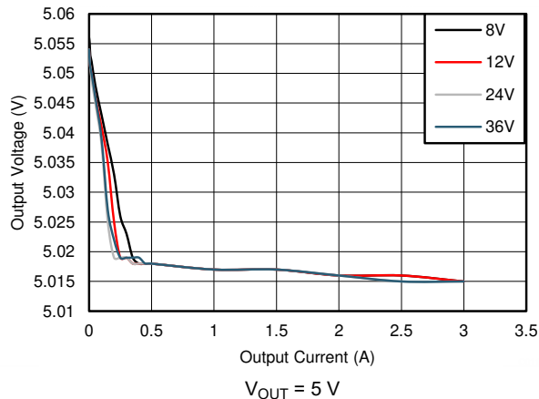
8-11. Line and Load Regulation
