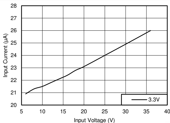
FIG 8-4. No-load Input Supply Current for 3.3-V Fixed Output Option
