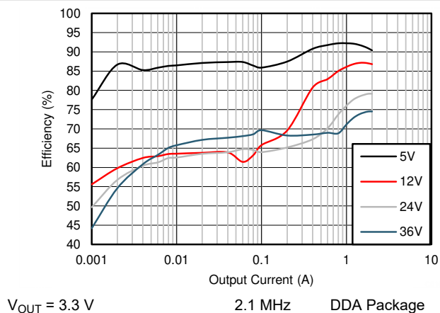
Figure 9-12. Efficiency
