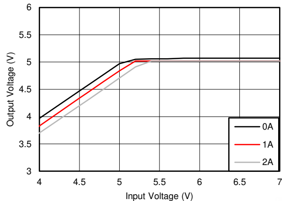
8-9. Overall Dropout Characteristic V_{OUT} = 5\text{ V}
