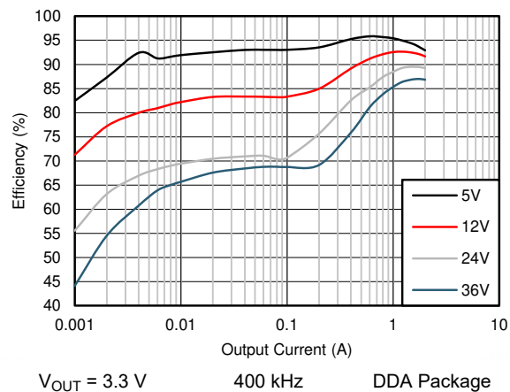
Figure 9-8. Efficiency
