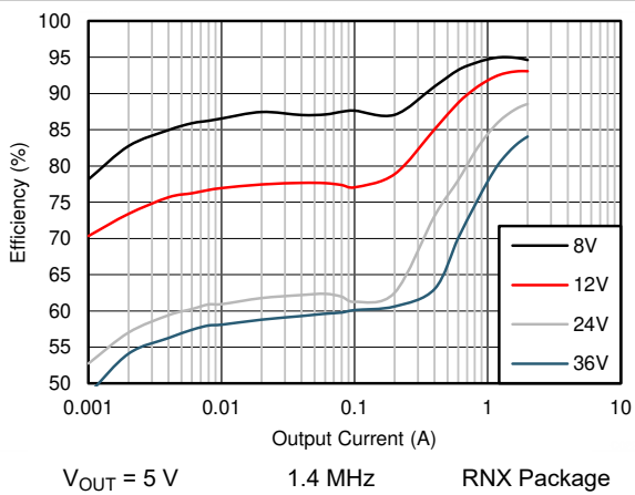
9-15. Efficiency
