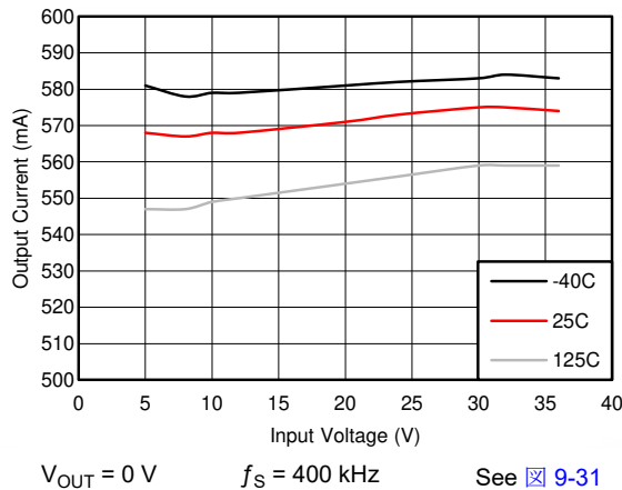
7-3. Short-Circuit Output Current
