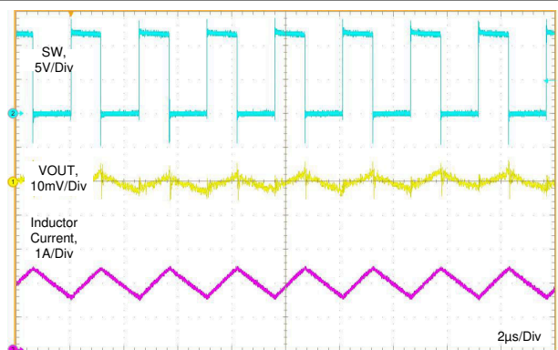
Figure 8-8. Typical PWM Switching Waveforms V_{IN} = 12 V, V_{OUT} = 5 V, I_{OUT} = 2 A, f_S = 400 kHz
