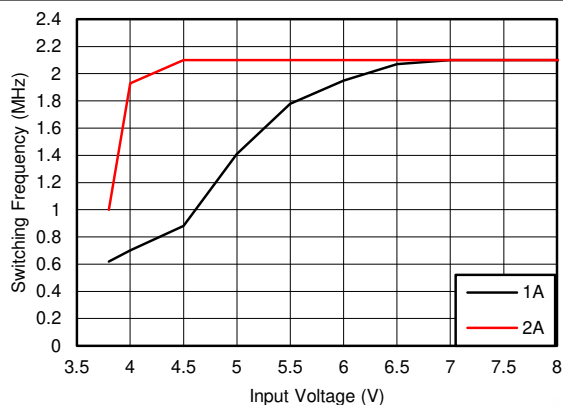
8-11. Typical Switching Frequency in Dropout Mode V_{OUT} = 3.3\text{ V} , f_{SW} = 2.1\text{ MHz}
