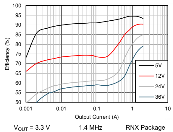
9-16. Efficiency
