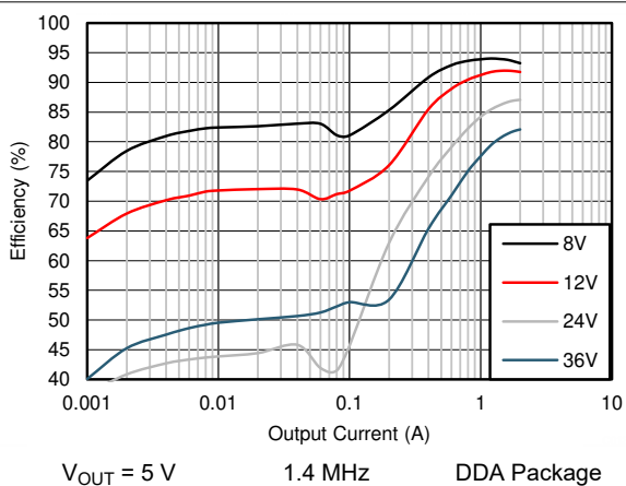
Figure 9-9. Efficiency
