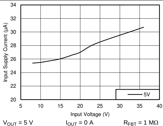
図 28. Input Supply Current
