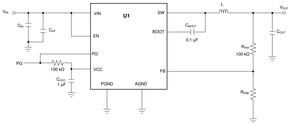
FIG 36. Circuit for Application Curves
