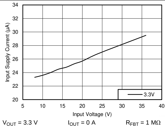
図 29. Input Supply Current
