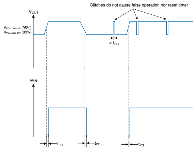
Figure 8. Power-Good-Timing Behavior
