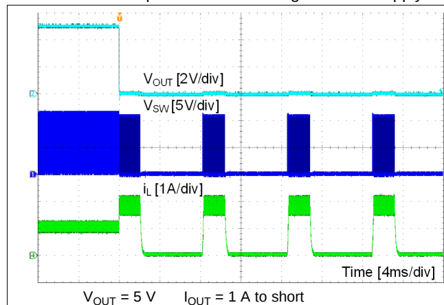
Figure 28. Short Protection
