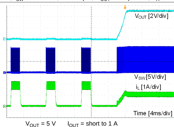
Figure 29. Short Recovery
