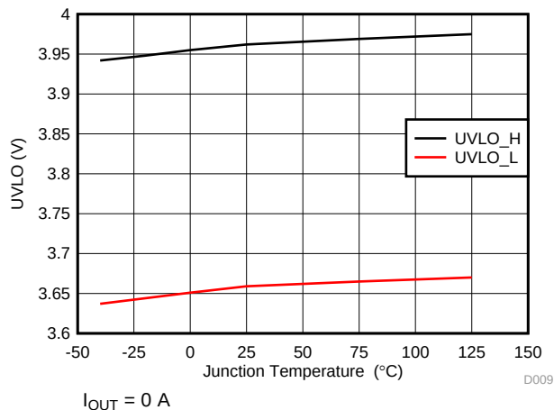
Figure 12. UVLO Threshold
