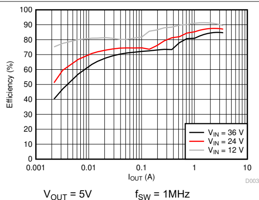
図 5-2. Efficiency vs. Load Current
