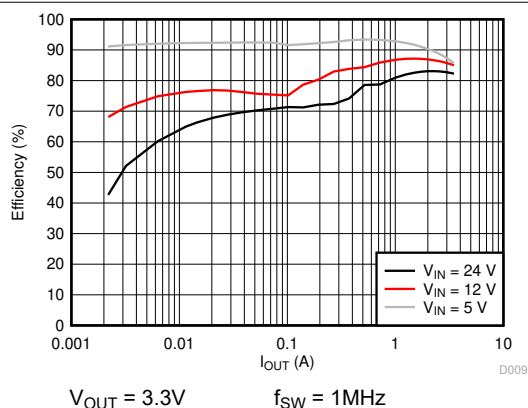
図 5-3. Efficiency vs. Load Current
