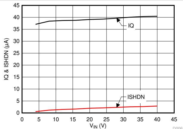
図 5-11. Shut-down Current and Quiescent Current
