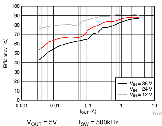
図 5-1. Efficiency vs. Load Current
