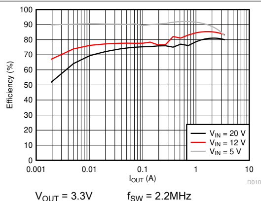
図 5-4. Efficiency vs. Load Current
