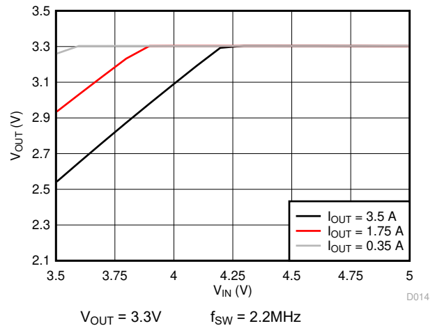
図 5-10. Dropout Curve
