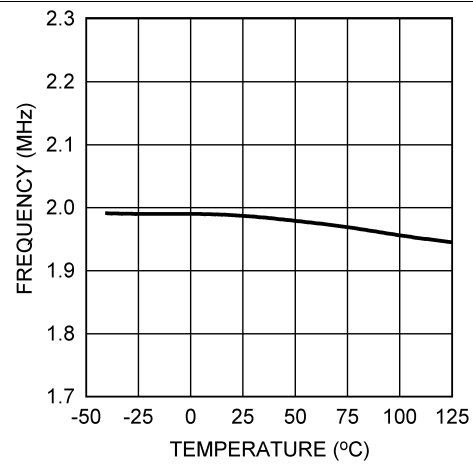
Figure 14. Oscillator Frequency vs Temperature
