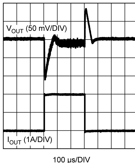
Figure 29. LMR12015/20 Load Transient Without C_{FF} Capacitor V_{OUT} = 3.3 V
