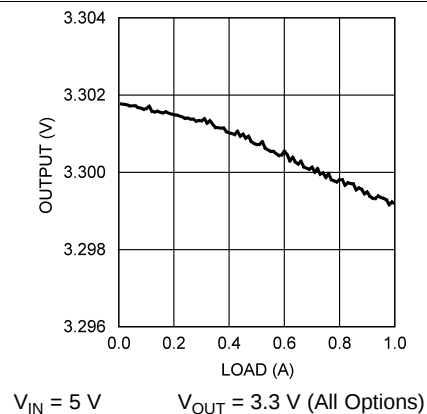
Figure 20. Load Regulation
