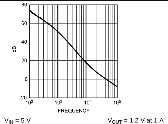
Figure 12. Gain vs Frequency
