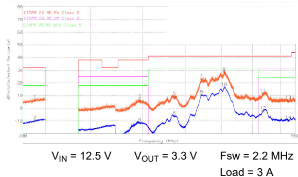
図 8-23. CISPR 25 Class 5 Radiated EMI, Log Antenna, Horizontal Polarization, 300 MHz - 960 MHz Orange: Peak Detect, Blue: Average Detect
