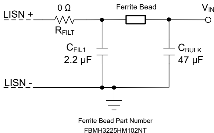
図 8-25. Typical Input EMI Filter
