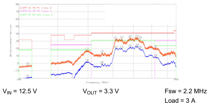
図 8-24. CISPR 25 Class 5 Radiated EMI, Log Antenna, Vertical Polarization, 300 MHz - 960 MHz Orange: Peak Detect, Blue: Average Detect
