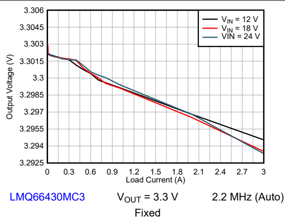
8-7. Line and Load Regulation
