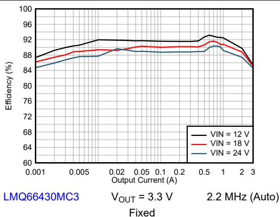
8-4. Efficiency
