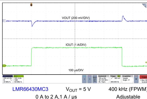
8-31. Load Transient
