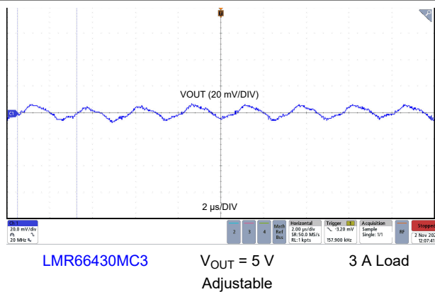
8-32. Output Voltage Ripple
