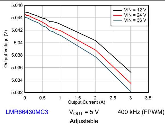
8-28. Line and Load Regulation
