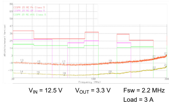
図 8-22. CISPR 25 Class 5 Radiated EMI, Biconical Antenna, Vertical Polarization, 30 MHz - 300 MHz Orange: Peak Detect, Yellow: Average Detect
