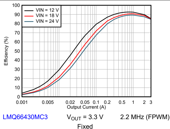
8-5. Efficiency
