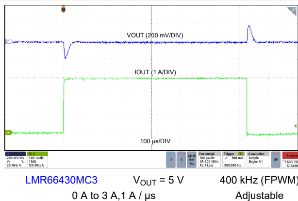
8-30. Load Transient
