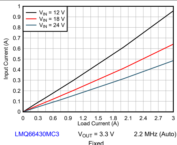
8-9. Input Current vs Load Current
