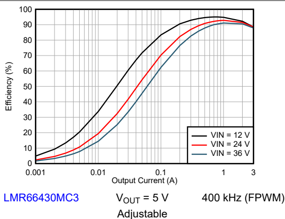
8-27. Efficiency
