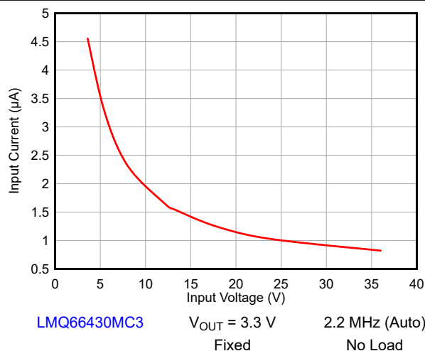
8-8. Input Switching Current vs Input Voltage
