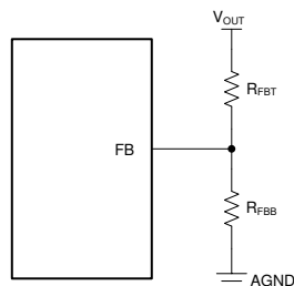
図 7-8. Setting Output Voltage for Adjustable Output Variant
