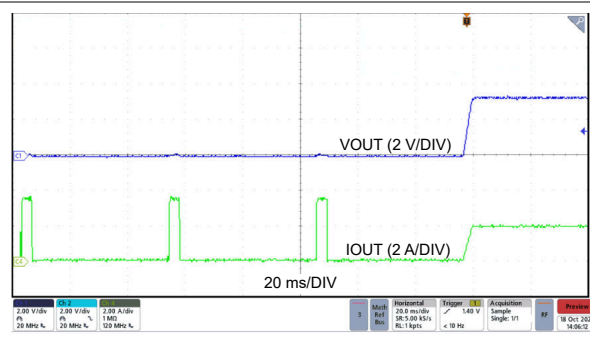
8-12. Hiccup Exit
