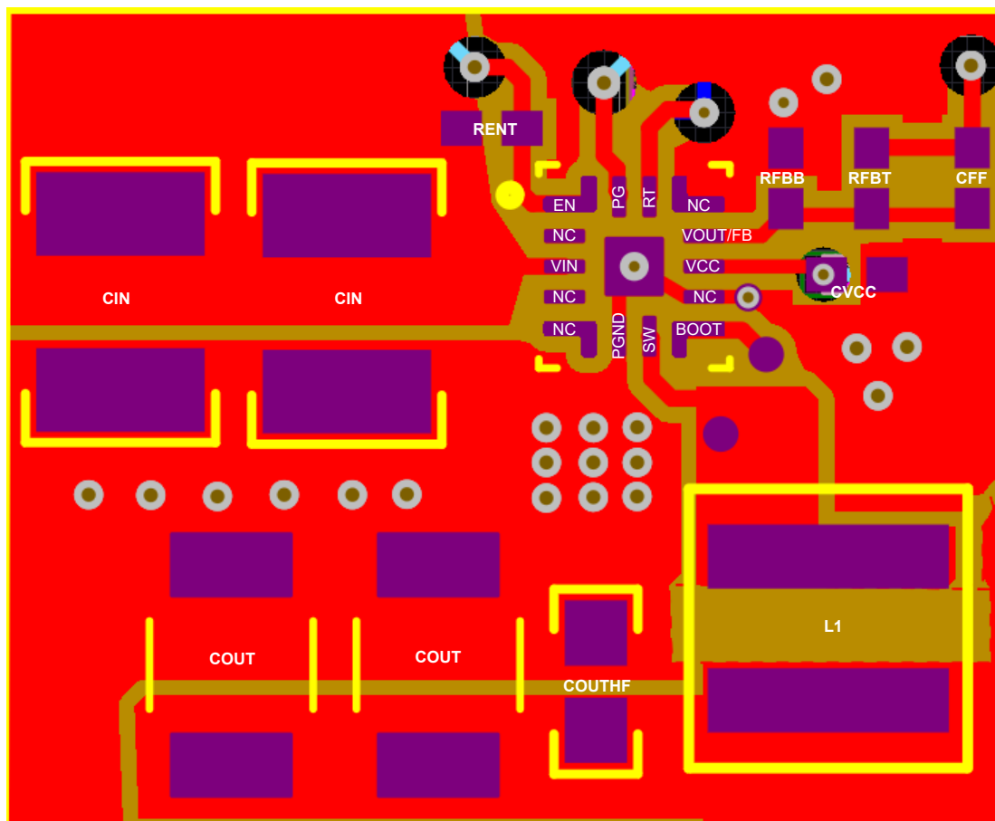
9-13. Example Layout
