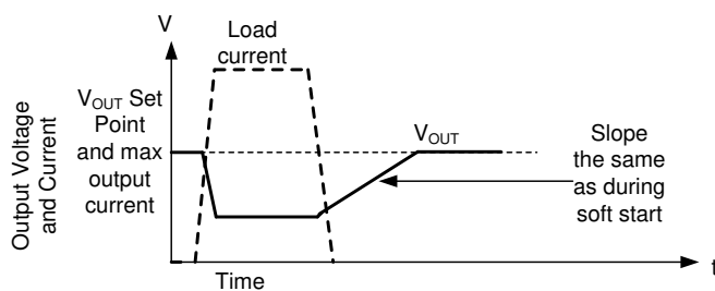
8-8. Recovery from Dropout
