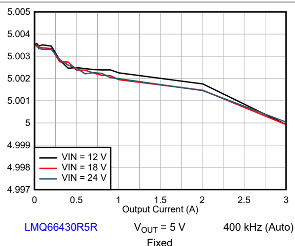
9-7. Line and Load Regulation
