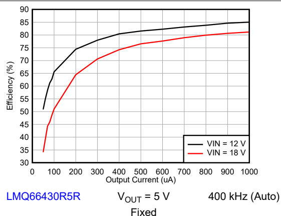
9-5. Efficiency
