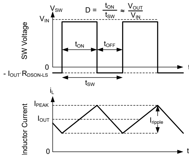
8-13. SW Voltage and Inductor Current Waveforms in Continuous Conduction Mode (CCM)
