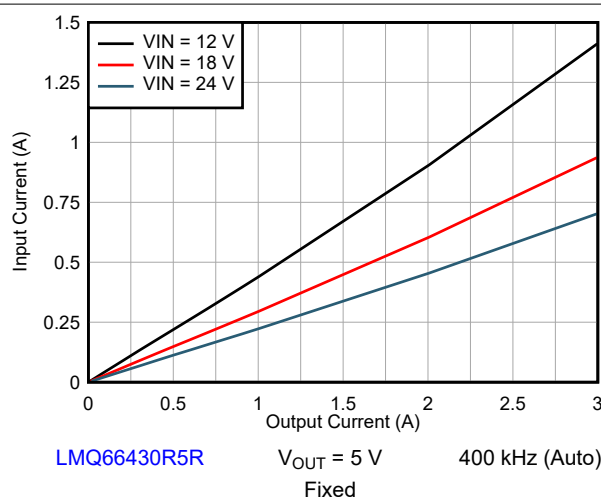
9-6. Input Current vs Load Current
