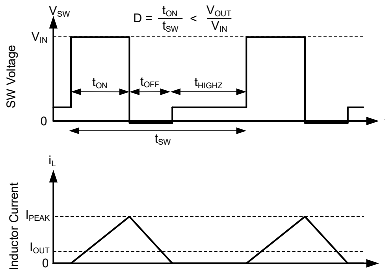
Figure 8-14. PFM Operation
