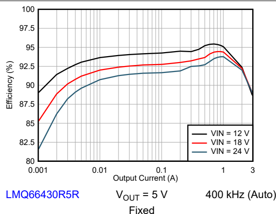
9-4. Efficiency
