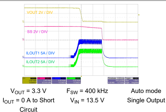
図 8-41. Short-Circuit Protection
