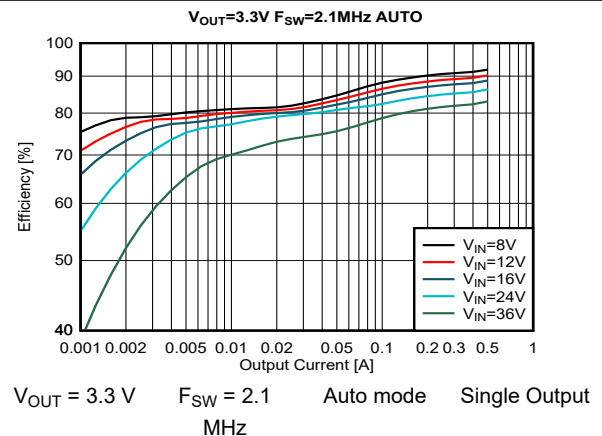
図 8-18. Efficiency
