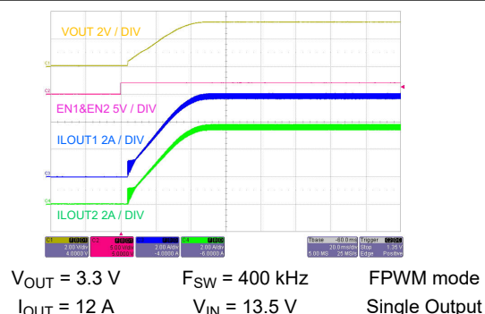
図 8-40. Start-Up With 12-A Load
