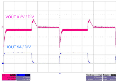
V_{OUT} = 5\text{ V} F_{SW} = 400\text{ kHz} Auto mode I_{OUT} = 100\text{ mA to }6\text{ A to }100\text{ mA} V_{IN} = 13.5\text{ V} Dual Output
