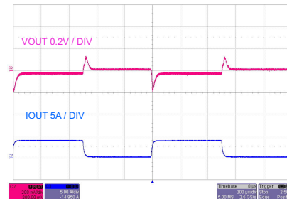
V_{OUT} = 3.3\text{ V} F_{SW} = 2.1\text{ MHz} Auto mode I_{OUT} = 100\text{ mA to }6\text{ A to }100\text{ mA} V_{IN} = 13.5\text{ V} Dual Output
