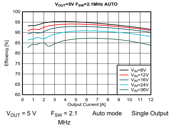
図 8-16. Efficiency
