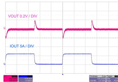
V_{OUT} = 5\text{ V} F_{SW} = 400\text{ kHz} FPWM mode I_{OUT} = 100\text{ mA to }6\text{ A to }100\text{ mA} V_{IN} = 13.5\text{ V} Dual Output
