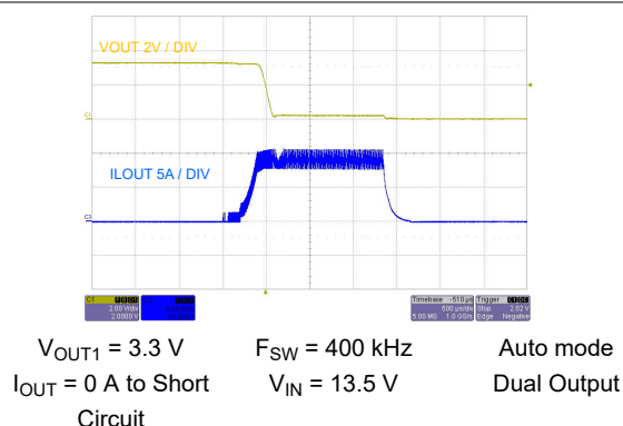
図 8-42. Short-Circuit Protection
