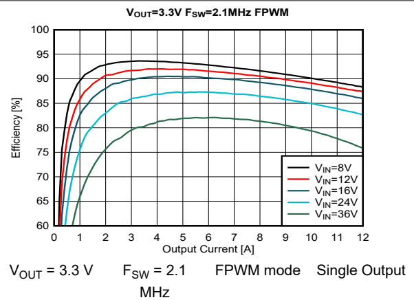
図 8-20. Efficiency
