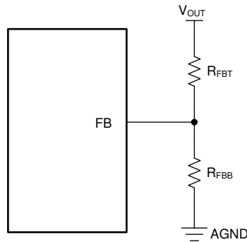
図 7-3. Setting Output Voltage of Adjustable Versions
