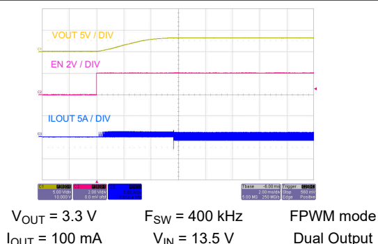
図 8-39. Start-Up With 100-mA Load
