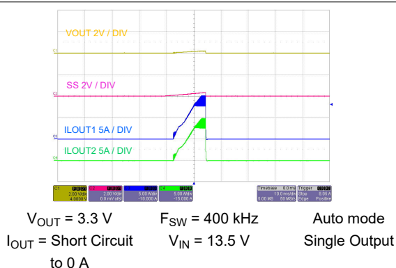
図 8-43. Short-Circuit Hiccup
