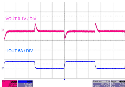
V_{OUT} = 3.3\text{ V} F_{SW} = 2.1\text{ MHz} FPWM mode I_{OUT} = 100\text{ mA to }6\text{ A to }100\text{ mA} V_{IN} = 13.5\text{ V} Dual Output
