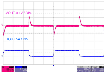
V_{OUT} = 5\text{ V} F_{SW} = 2.1\text{ MHz} FPWM mode I_{OUT} = 100\text{ mA to }6\text{ A to }100\text{ mA} V_{IN} = 13.5\text{ V} Dual Output
