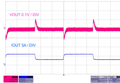
V_{OUT} = 5\text{ V} F_{SW} = 400\text{ kHz} FPWM mode I_{OUT} = 3\text{ A to }6\text{ A to }3\text{ A} V_{IN} = 13.5\text{ V} Dual Output
