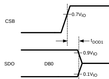
Figure 7. SDO and \overline{CS} Timing
