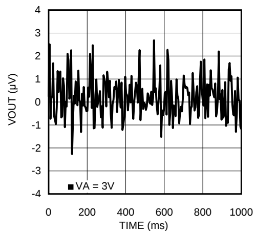
Figure 21. Noise Measurement With Calibration at Gain = 128
