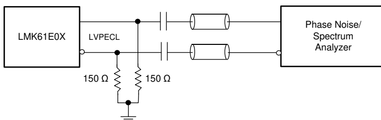
7-4. LVPECL Output AC Configuration During Device Test
