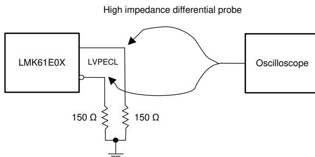
7-1. LVPECL Output DC Configuration During Device Test
