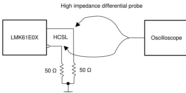
7-2. LVDS Output DC Configuration During Device Test
