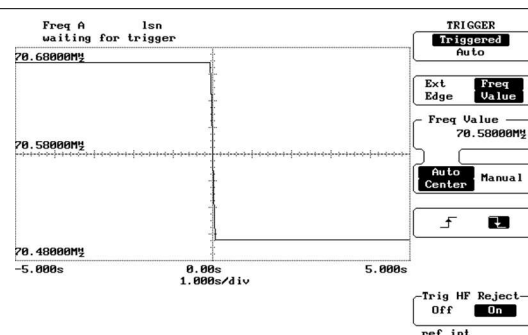
✎ 9-3. Decreasing Output Frequency in DCXO Mode
