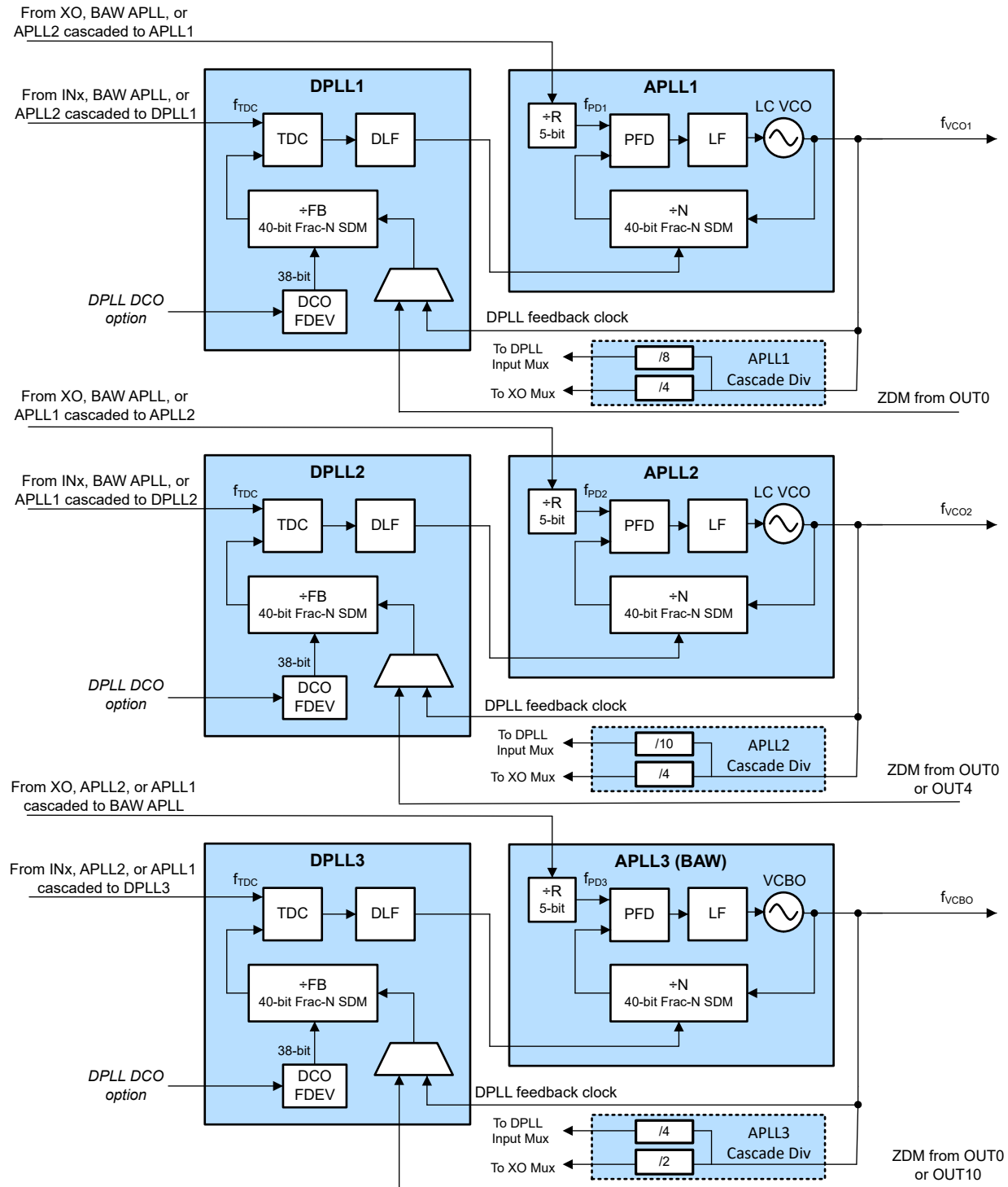
図 8-2. PLL Architecture
