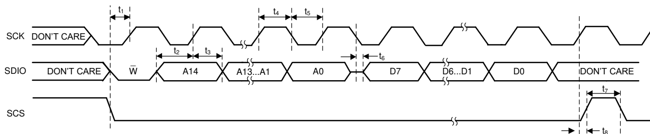
図 6-3. SPI 3-Wire Read Timing Diagram
