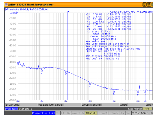
図 6-9. 245.76MHz HS Output From BAW APLL
