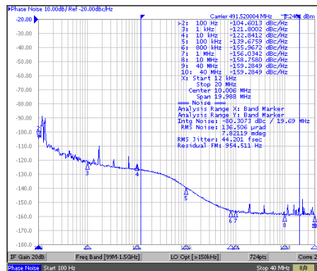
図 6-8. 491.52MHz HS Output From BAW APLL
