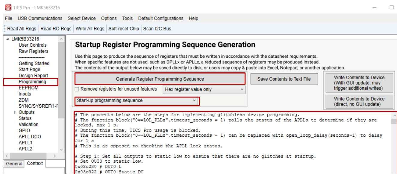
Figure 7-46. LMK5xxxxxx TICS Pro Programming Page (Screenshot From v1.7.7.4.)
