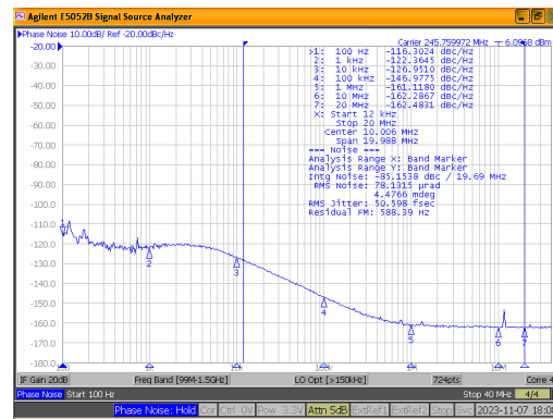
図 5-9. 245.76MHz HSDDS Output From APLL1 BAW
