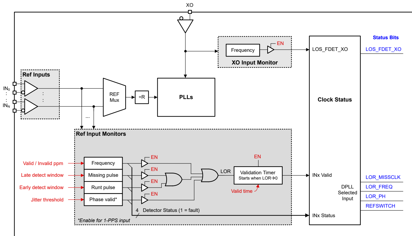
图 7-16. Clock Monitors for Reference and XO Inputs
