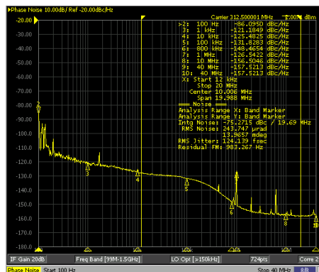
図 5-12. 312.5MHz HSDDS Output From APLL2
