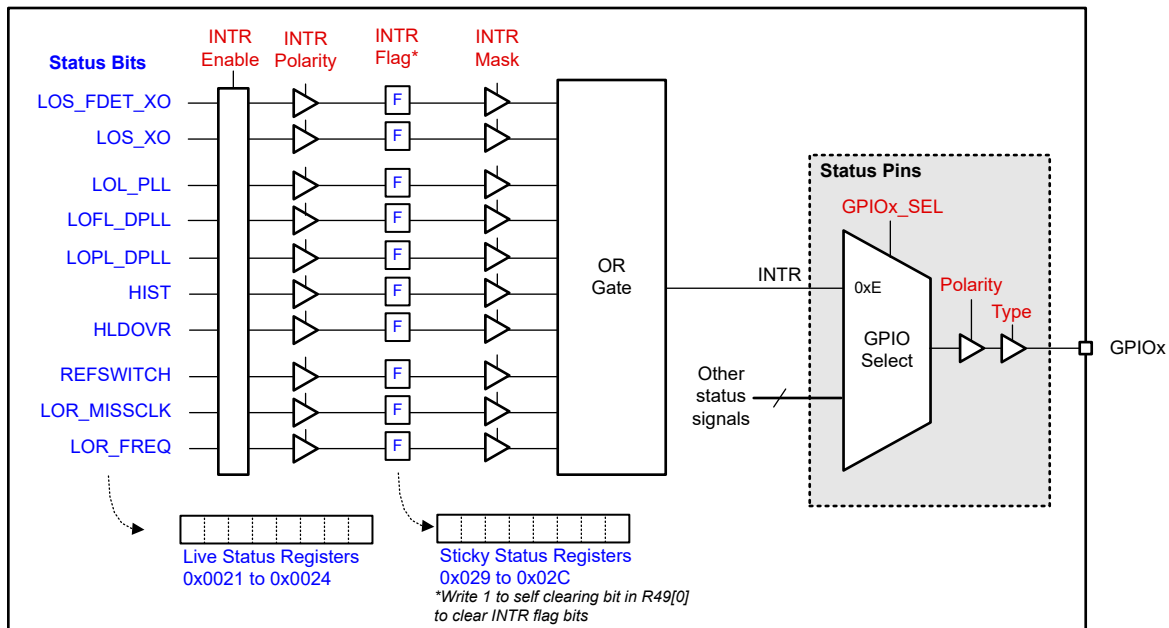
图 8-22. Status and Interrupt
