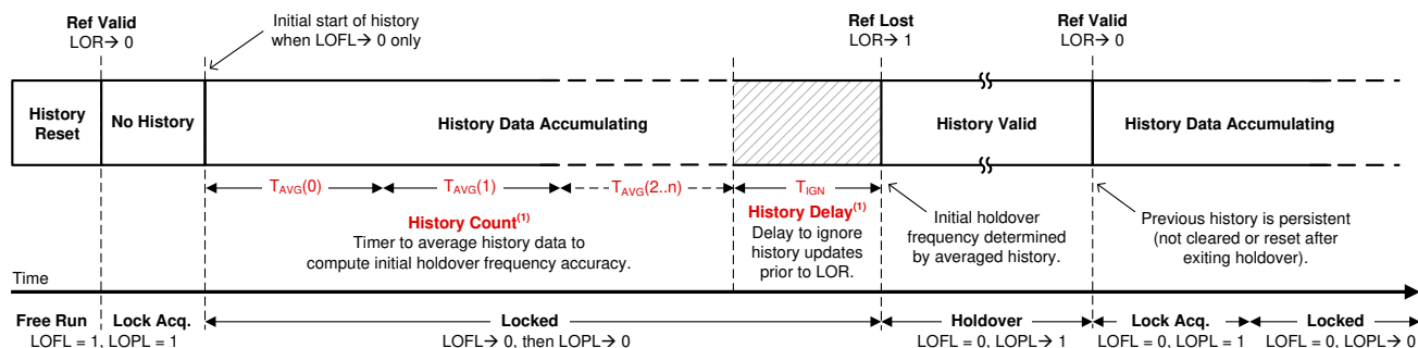
FIG 9-20. Tuning Word History Windows
