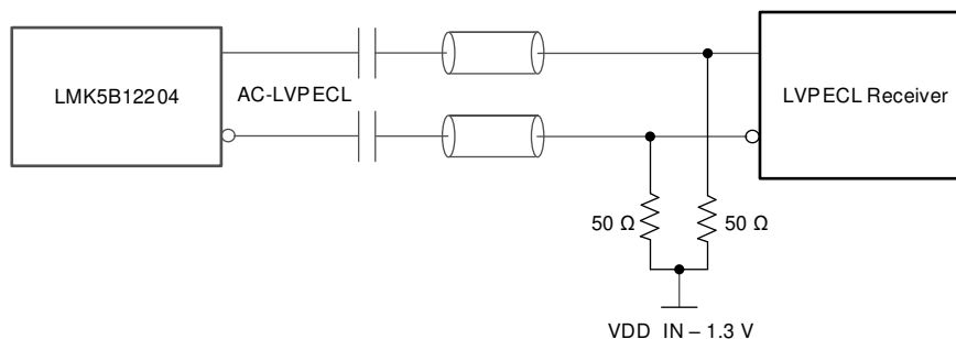
9-28. AC-CML Output to CML Receiver With Internal Termination/Biasing
