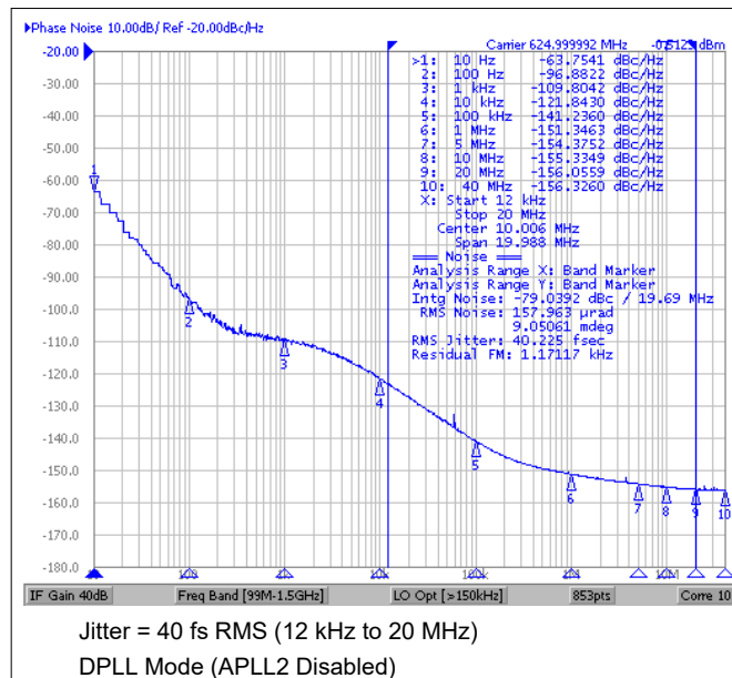
Figure 7-5. 625-MHz Output Phase Noise (APLL1)
