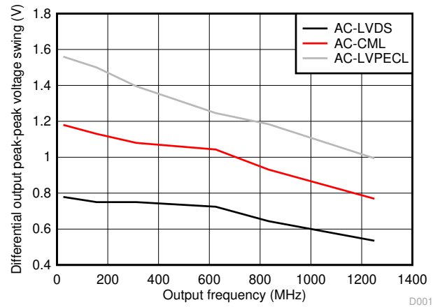
7-13. Output Swing vs Frequency
