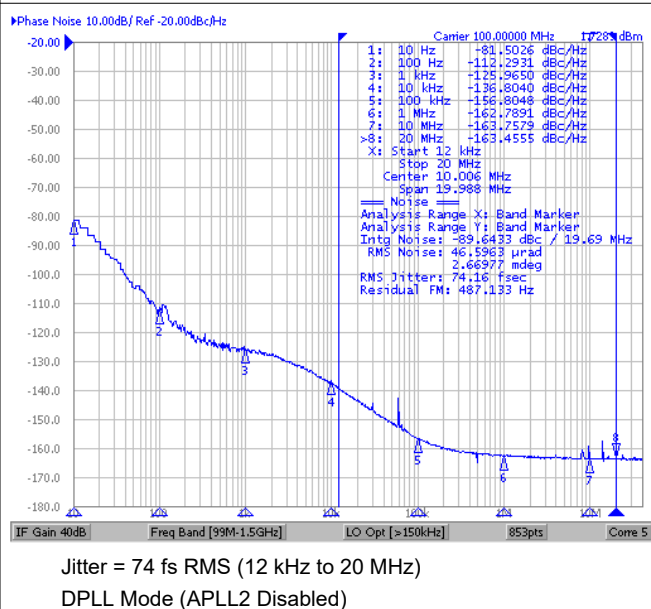
Figure 7-8. 100-MHz Output Phase Noise (APLL1)
