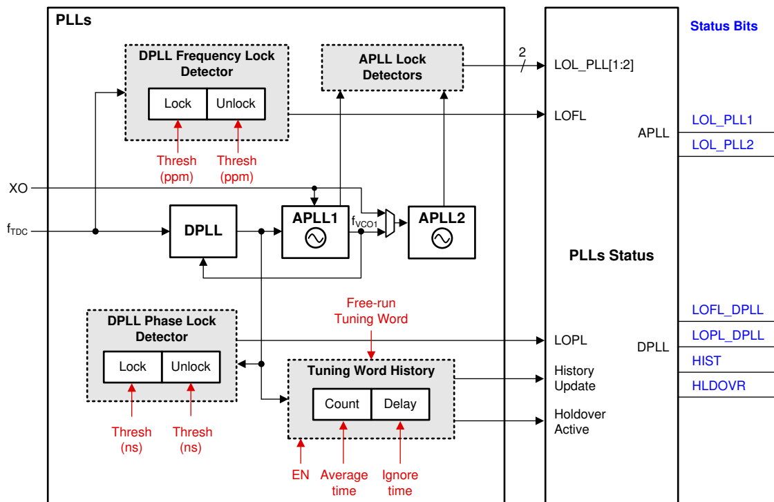
9-19. PLL Lock Detectors and History Monitor
