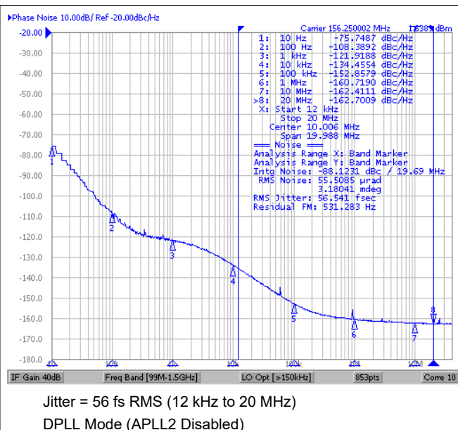
Figure 7-6. 156.25-MHz Output Phase Noise (APLL1)
