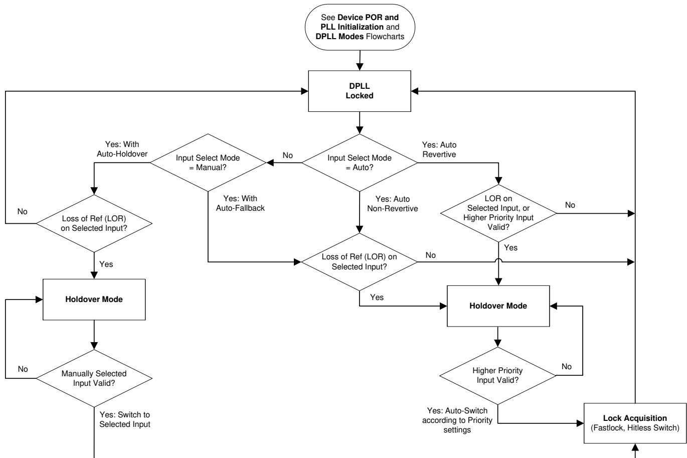
FIG 9-15. Reference Input Selection Flowchart
