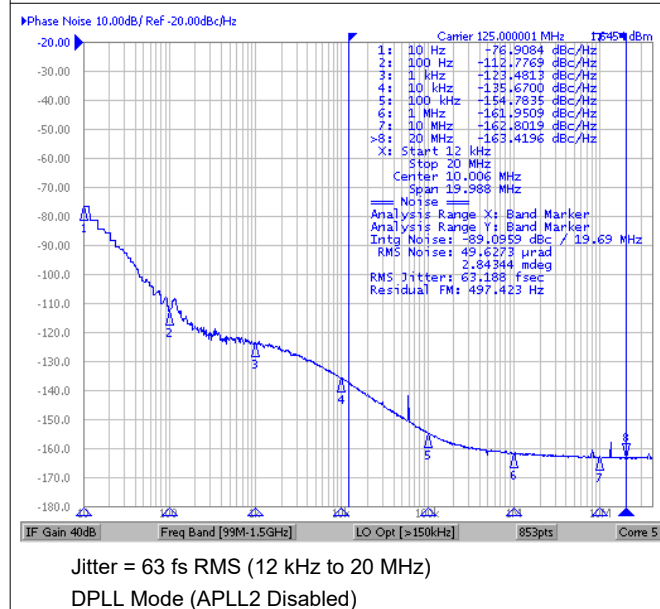
Figure 7-7. 125-MHz Output Phase Noise (APLL1)
