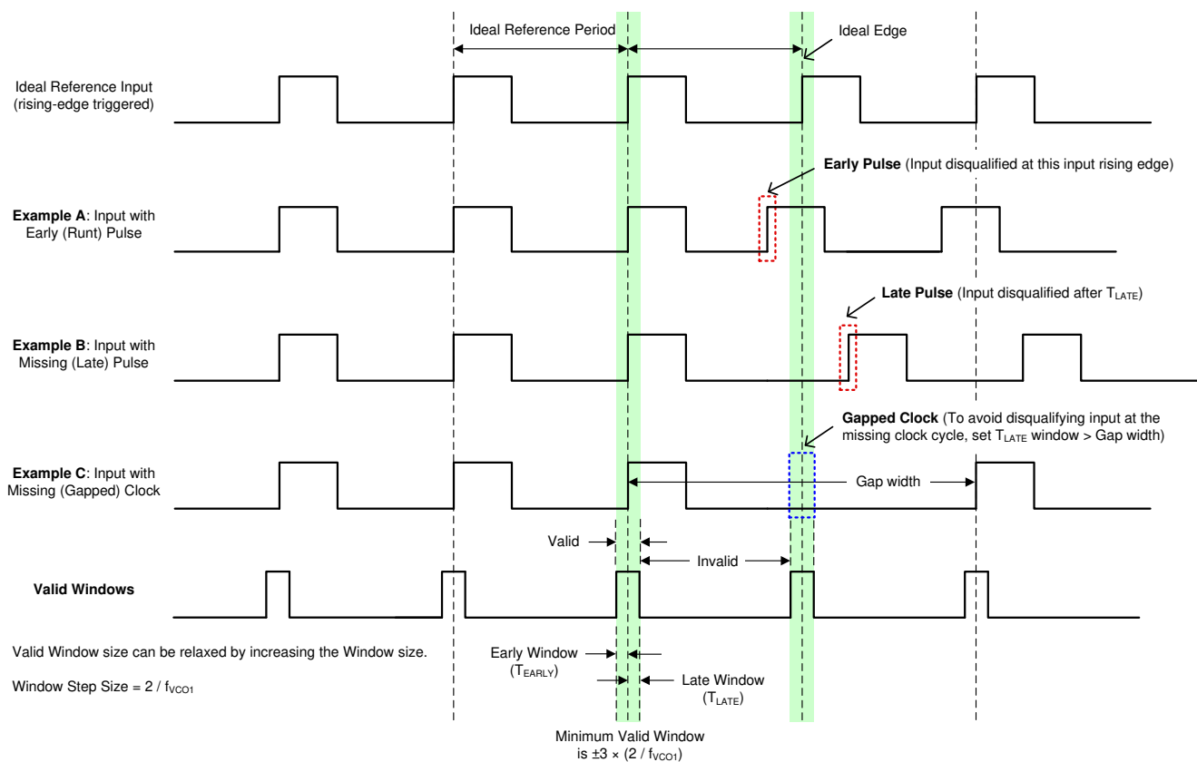
FIG 9-17. Early and Late Window Detector Examples
