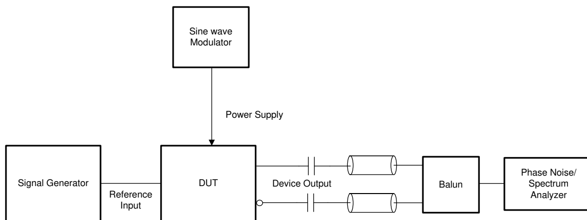
8-6. HCSL Output Phase Noise Test Configuration
