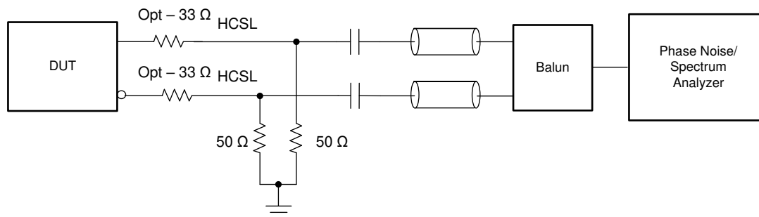
8-6. HCSL Output Phase Noise Test Configuration
