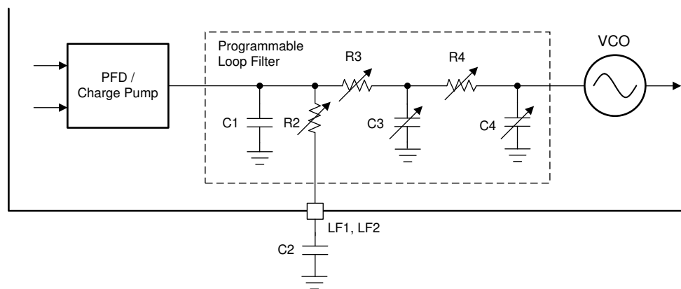
図 9-23. Loop Filter Structure of Each APLL
