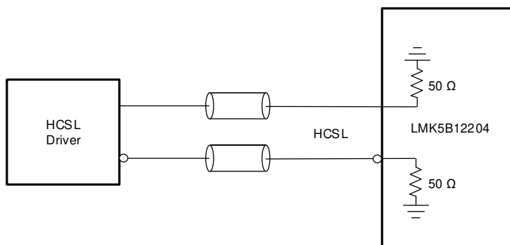
9-12. DC-Coupled CML (Source Terminated) to Reference (PRIREF/SECREP) or XO Inputs
