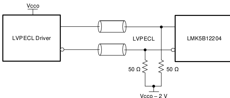
9-10. DC-Coupled LVPECL to Reference (PRIREF_P/SECREP_P) or XO Inputs
