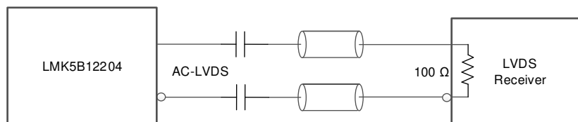
9-27. AC-LVDS Output to LVDS Receiver With Internal Termination/Biasing
