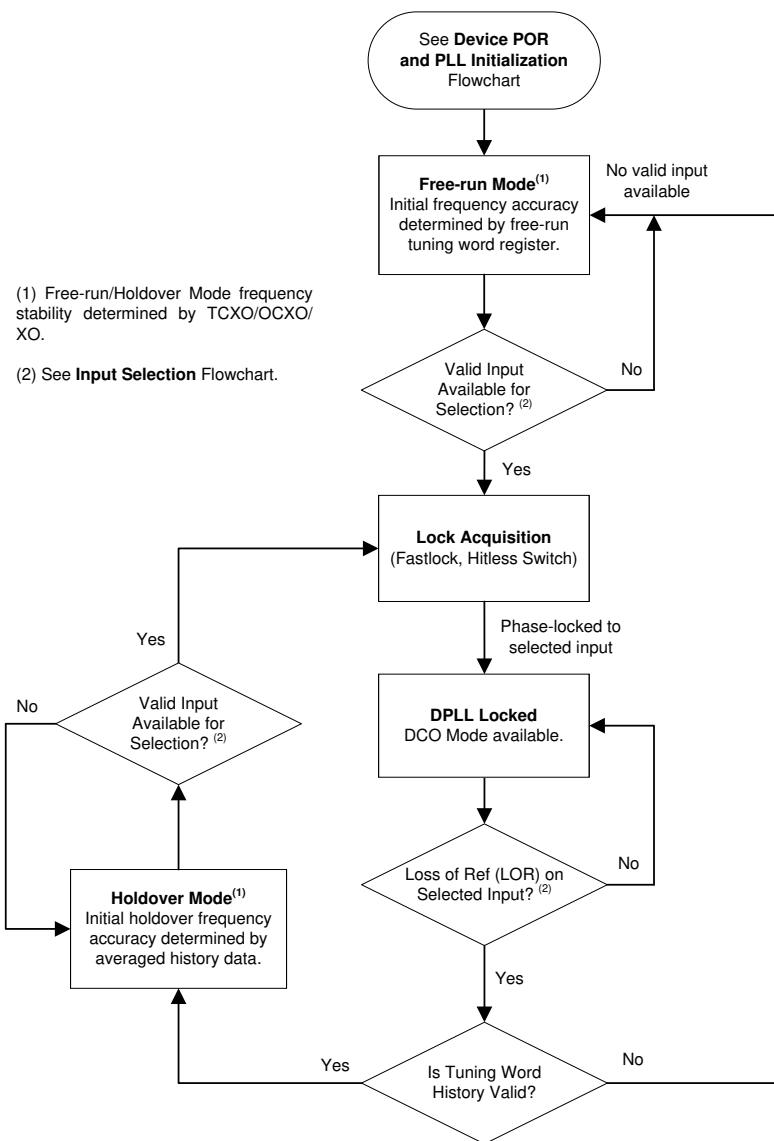
9-32. PLL Operating Mode
