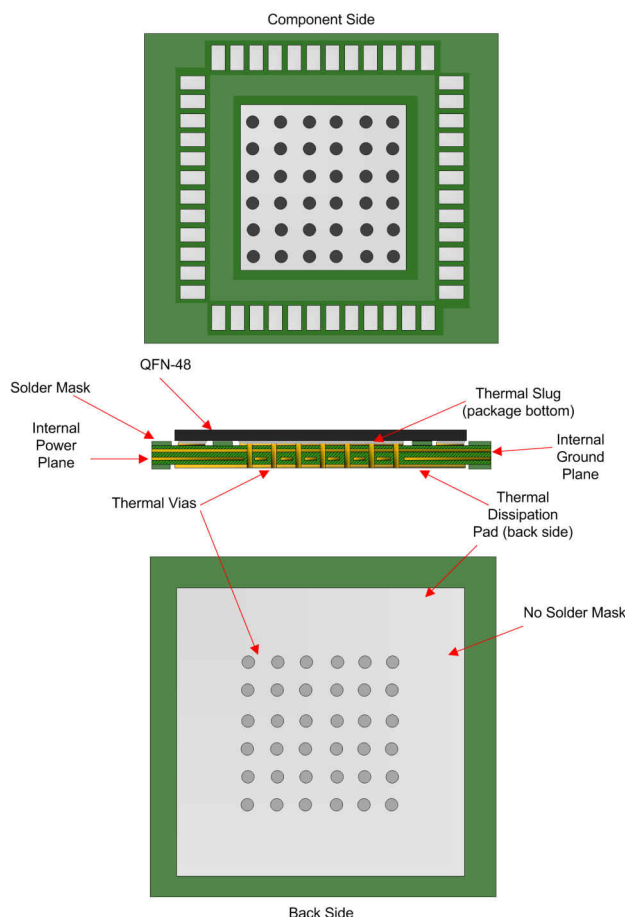
図 12-1. General PCB Ground Layout for Thermal Reliability (8+ Layers Recommended)
