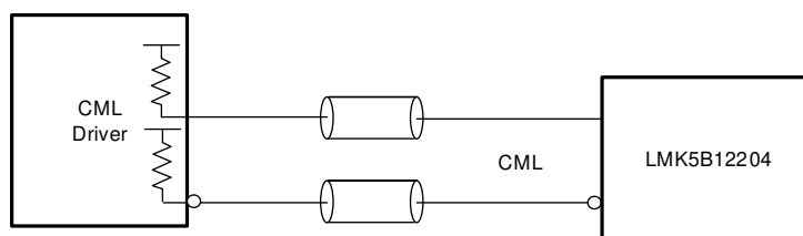
9-11. DC-Coupled LVDS to Reference (PRIREF/SECREP) or XO Inputs
