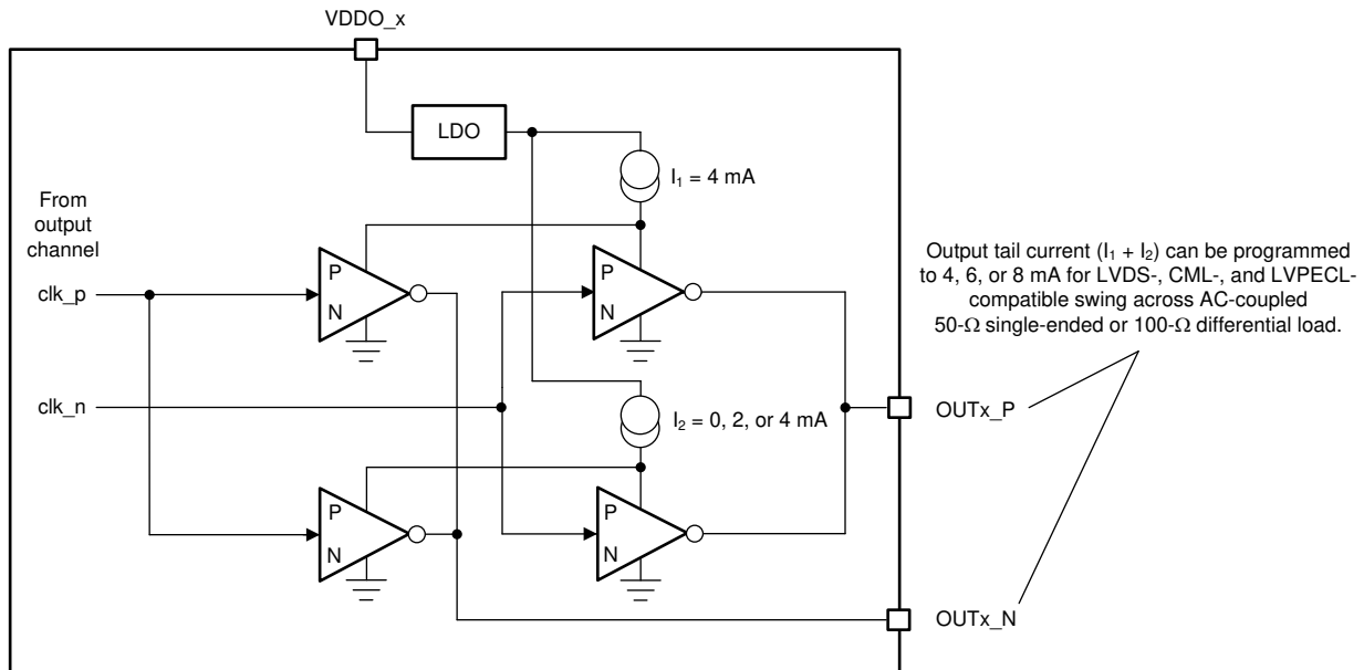
FIG 9-25. AC-LVDS/CML/LVPECL Output Driver Structure
