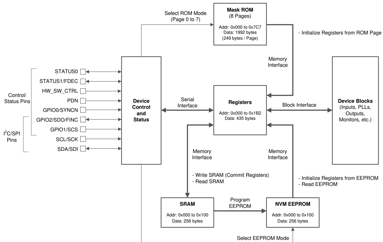
FIG 9-35. Device Control, Register, and Memory Interfaces
