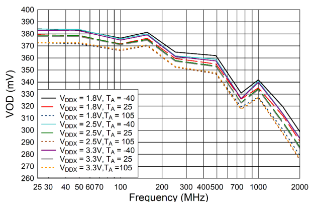
図 6-9. LMK1D210xL VOD vs. Frequency, AMP_SELA / AMP_SELB = 0
