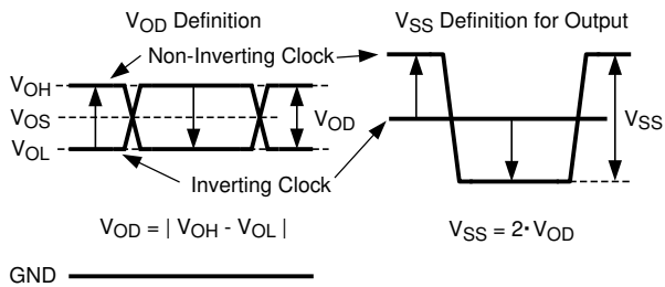
図 7-9. Two Different Definitions for Differential Output Signals
