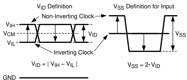
図 7-8. Two Different Definitions for Differential Input Signals
