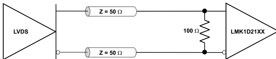
図 8-5. LVDS Clock Driver Connected to LMK1D210xL Input (DC-Coupled)
