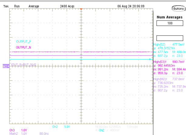
図 6-12. LMK1D210xL DC Output Common Mode at 1.8V Supply Condition, Differential Low (AMP_SELA / AMP_SELB = Float)
