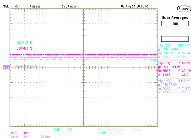
図 6-11. LMK1D210xL DC Output Common Mode at 1.8V Supply Condition, Differential Low (AMP_SELA / AMP_SELB = 0)
