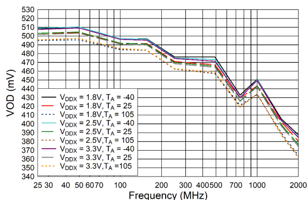
図 6-10. LMK1D210xL VOD vs. Frequency, AMP_SELA / AMP_SELB = Floating
