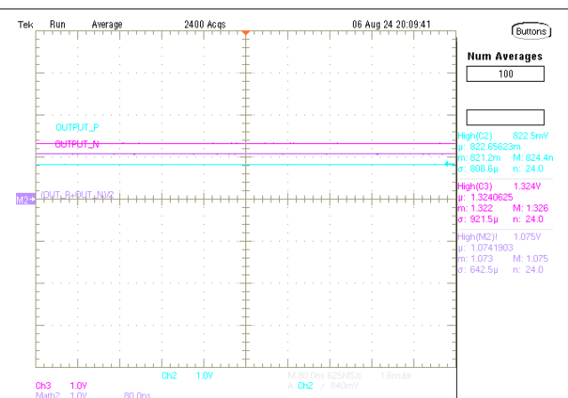
図 6-14. LMK1D210xL DC Output Common Mode at 2.5V/3.3V Supply Condition, Differential Low (AMP_SELA / AMP_SELB = Float)
