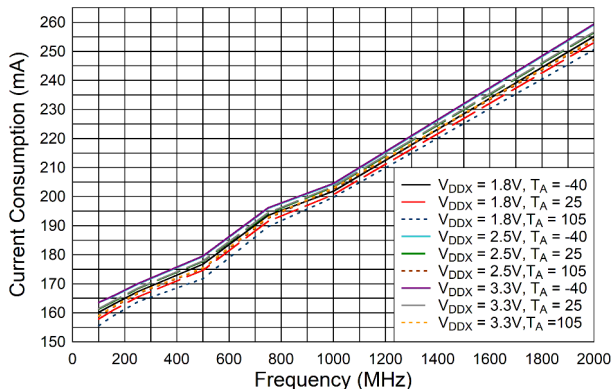
図 6-8. LMK1D2108L Current Consumption vs. Frequency, AMP_SELA and AMP_SELB = Floating
