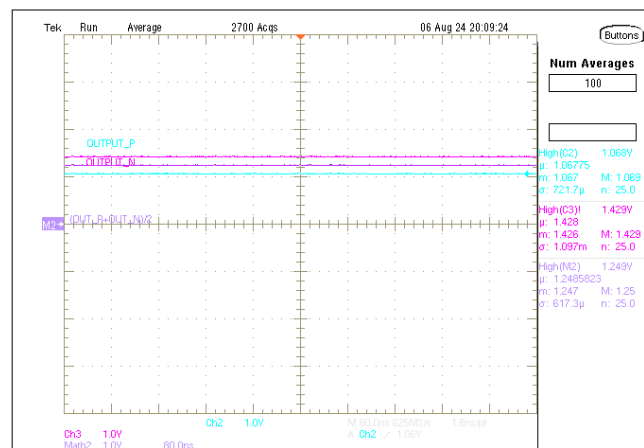
図 6-13. LMK1D210xL DC Output Common Mode at 2.5V/3.3V Supply Condition, Differential Low (AMP_SELA / AMP_SELB = 0)
