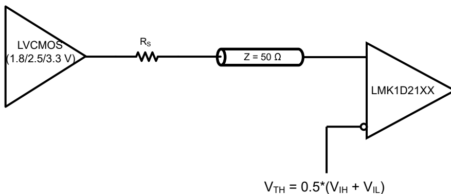
図 8-8. 1.8V, 2.5V, or 3.3V LVCMOS Clock Driver Connected to LMK1D210xL Input
