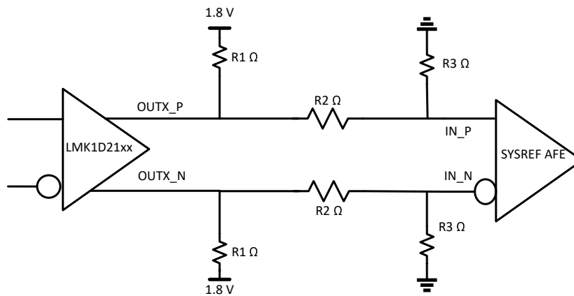
図 9-2. Schematic for DC-Coupling LMK1D210x With Lower Common-Mode Receiver
