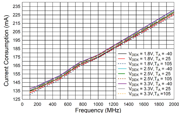
図 6-7. LMK1D2108L Current Consumption vs. Frequency, AMP_SELA and AMP_SELB = 0
