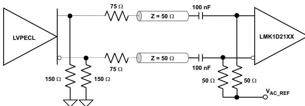
図 8-7. LVPECL Clock Driver Connected to LMK1D210xL Input
