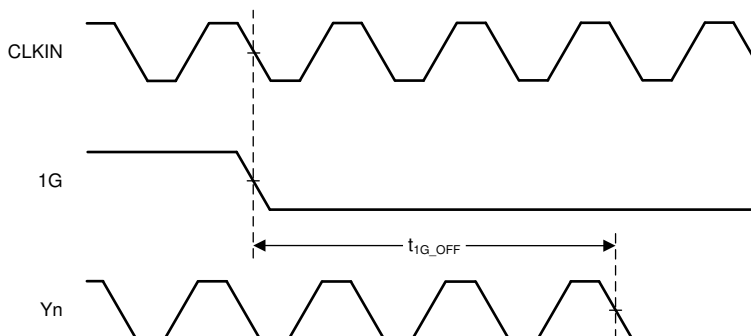
FIG 8-5. t_{1G\_OFF} Output Disable Time
