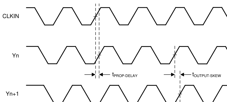
FIG 8-6. Propagation Delay t_{PROP-DELAY} and Output Skew t_{OUTPUT-SKEW}
