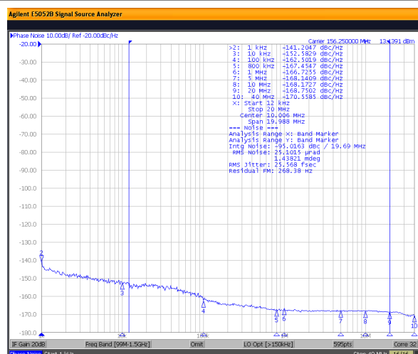
☒ 10-2. LMK1C110x Reference Phase Noise 25.6-fs (12 kHz to 20 MHz)
