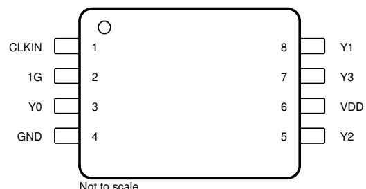
図 6-4. LMK1C1104 PW Package 8-Pin TSSOP Top View
