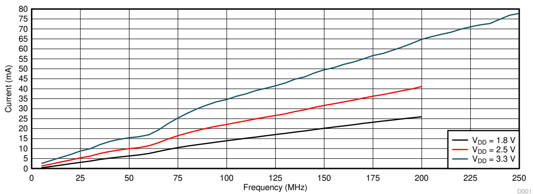
FIG 7-1. Device Power Consumption vs. Clock Frequency (Load 5 pF)
