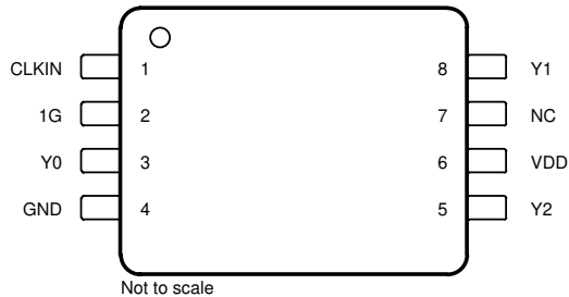
図 6-3. LMK1C1103 PW Package 8-Pin TSSOP Top View
