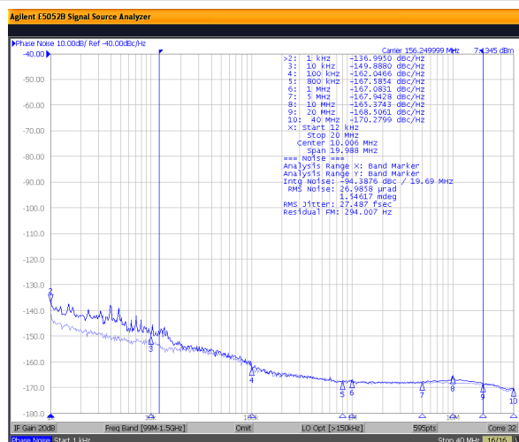
☒ 10-4. LMK1C110x 2.5-V Output Phase Noise 27.5-fs (12 kHz to 20 MHz)
