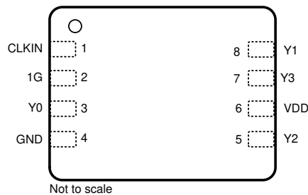
図 6-5. LMK1C1104 DQF Package 8-Pin WSON Top View
