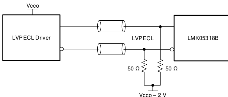
図 7-10. DC-Coupled LVPECL to Reference (PRIREF_P/SECREP_P) or XO Inputs
