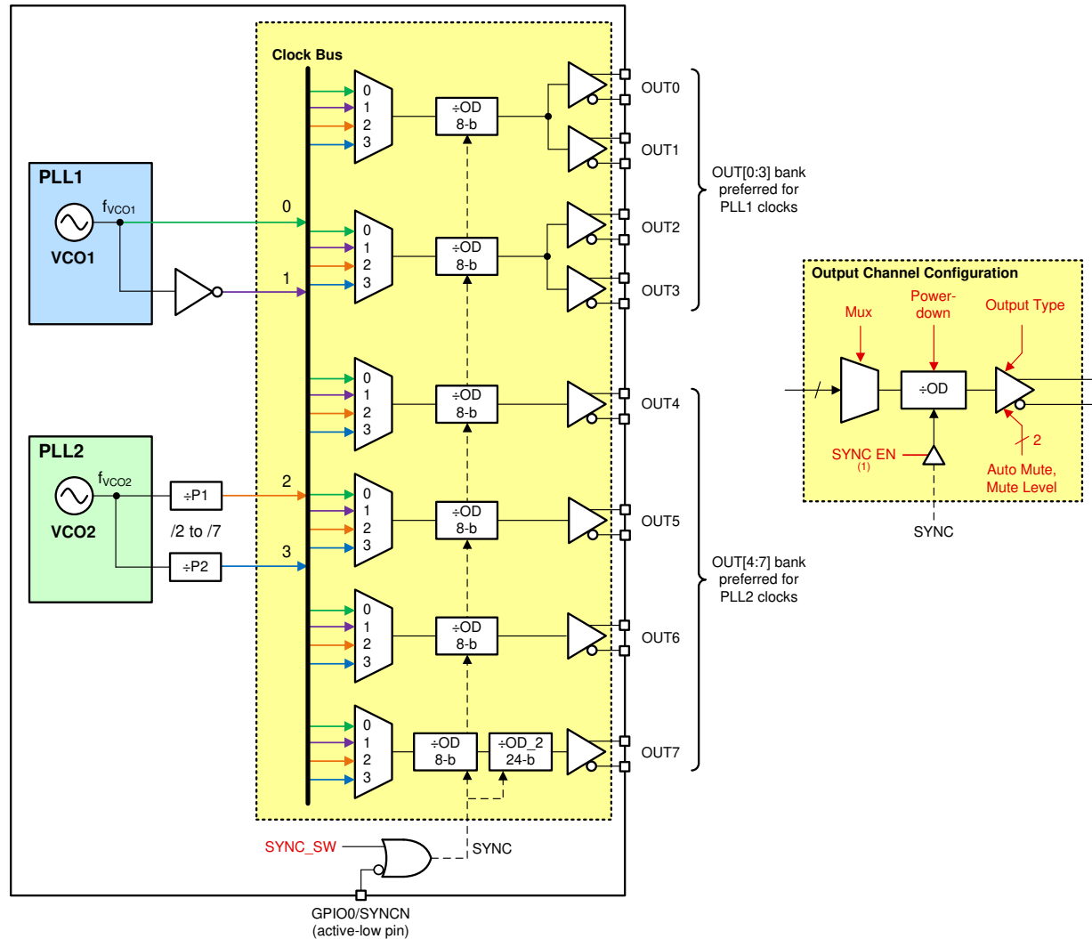
図 7-24. Output Clock Distribution
