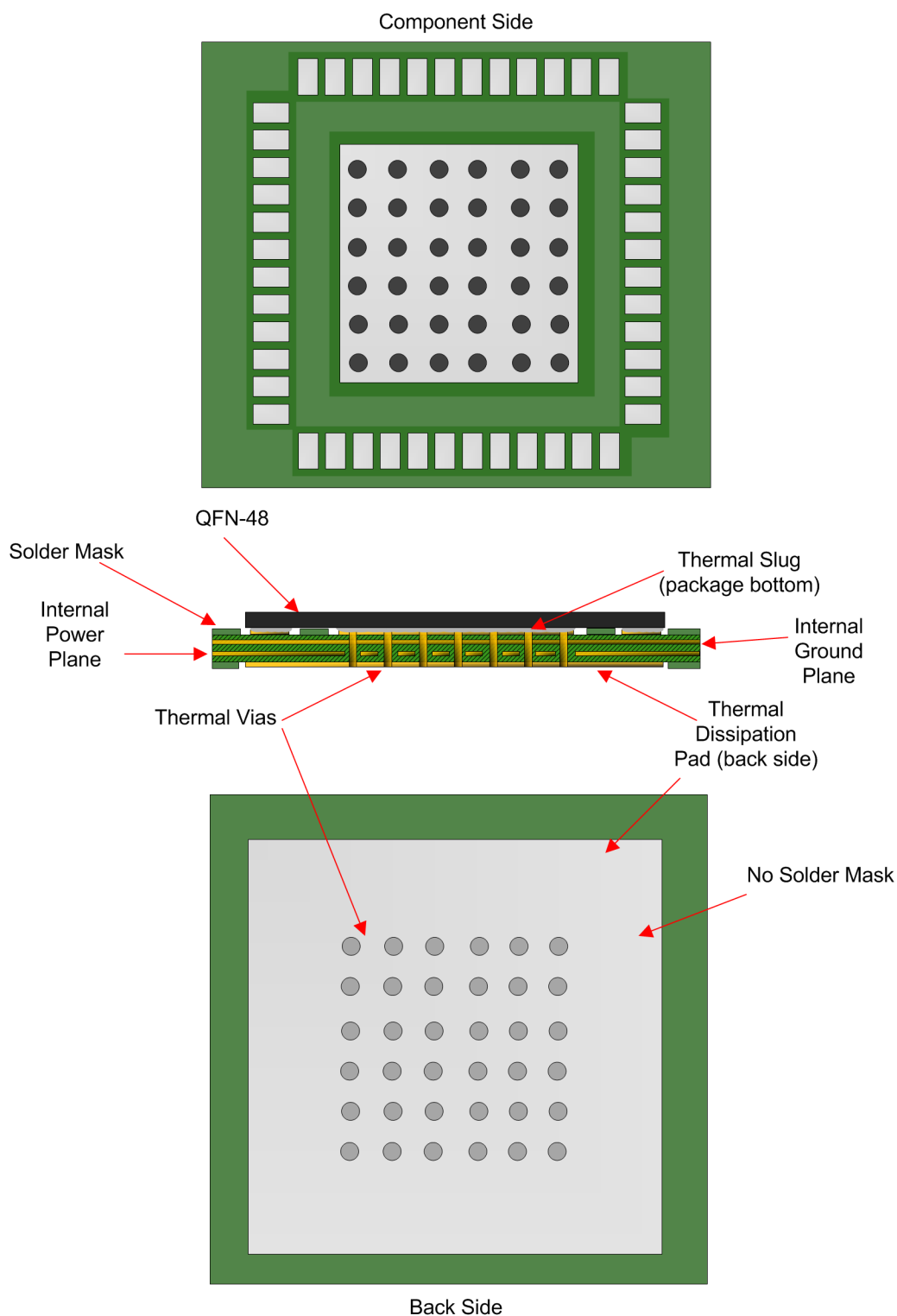
図 8-8. General PCB Ground Layout for Thermal Reliability (8+ Layers Recommended)
