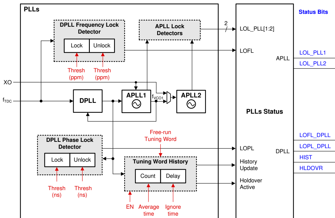
图 7-19. PLL Lock Detectors and History Monitor
