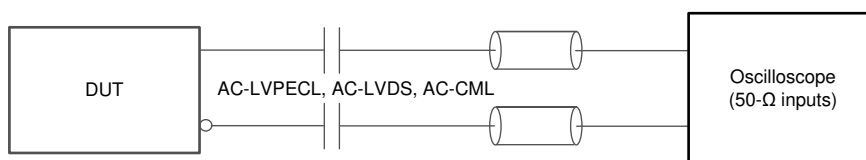
図 6-3. AC-LVPECL, AC-LVDS, AC-CML Output AC Test Configuration
