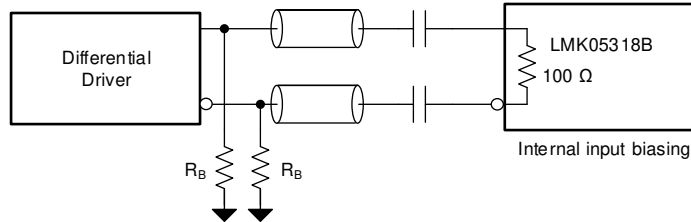
図 7-14. AC-Coupled Differential to Reference (PRIREF/SECREF) or XO Inputs
