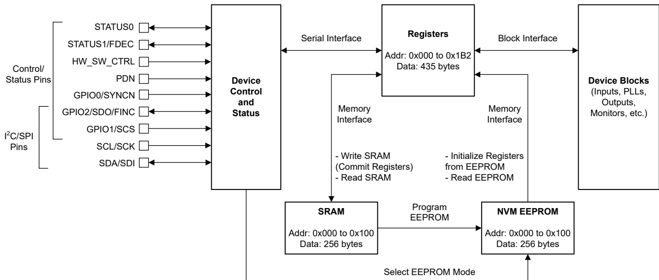
图 7-35. Device Control, Register, and Memory Interfaces
