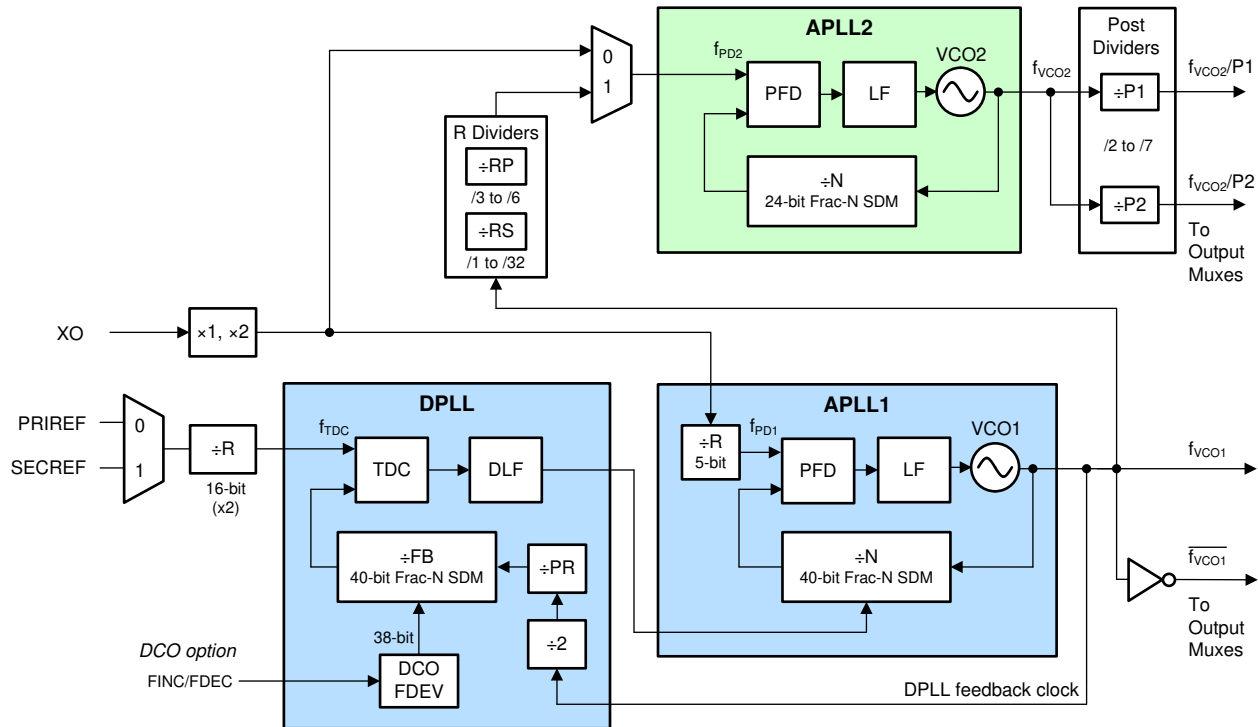
7-22. PLL Architecture
