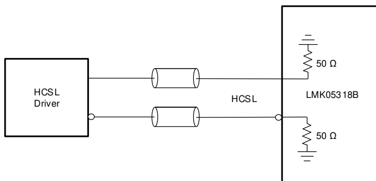
図 7-12. DC-Coupled CML (Source Terminated) to Reference (PRIREF/SECREP) or XO Inputs
