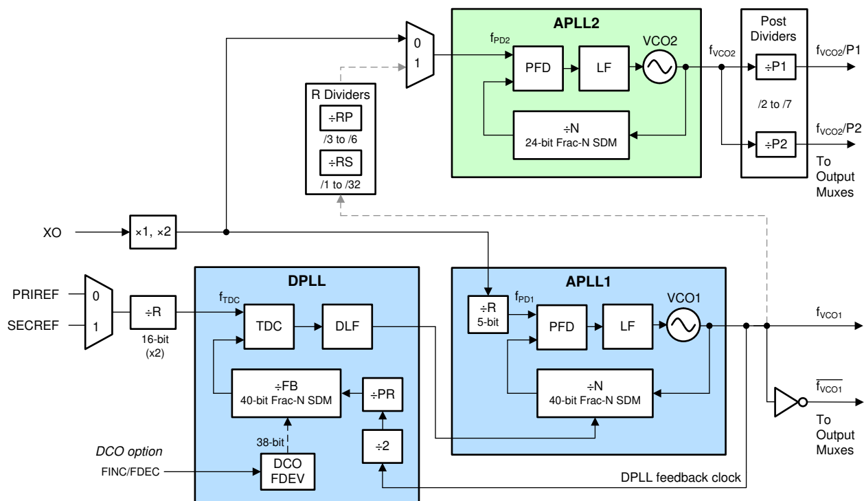
図 7-4. DPLL Mode With Non-Cascaded APLL2
