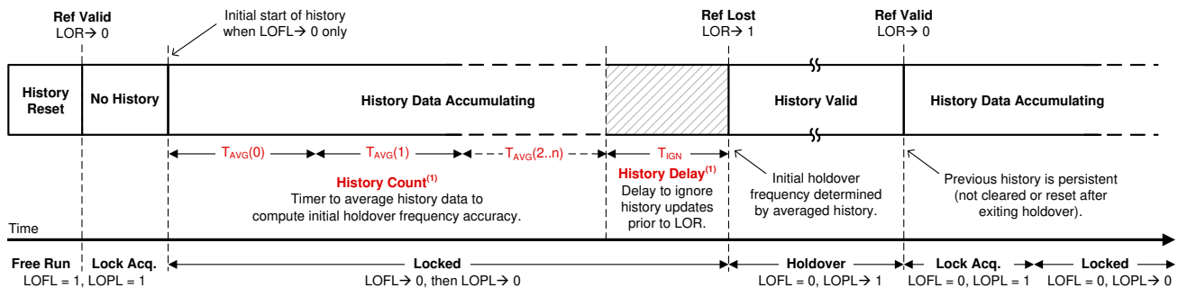
図 7-20. Tuning Word History Windows
