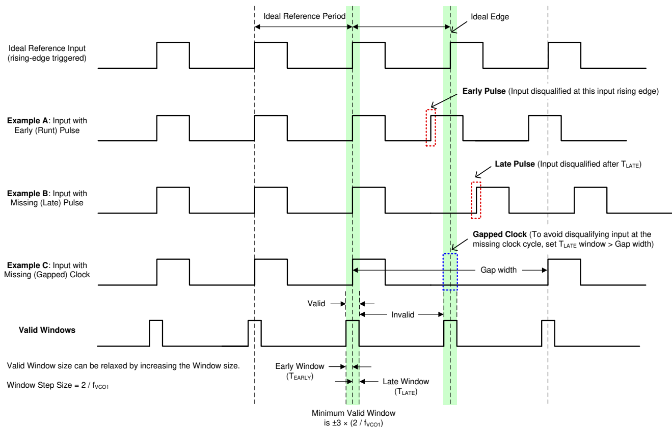
図 7-17. Early and Late Window Detector Examples
