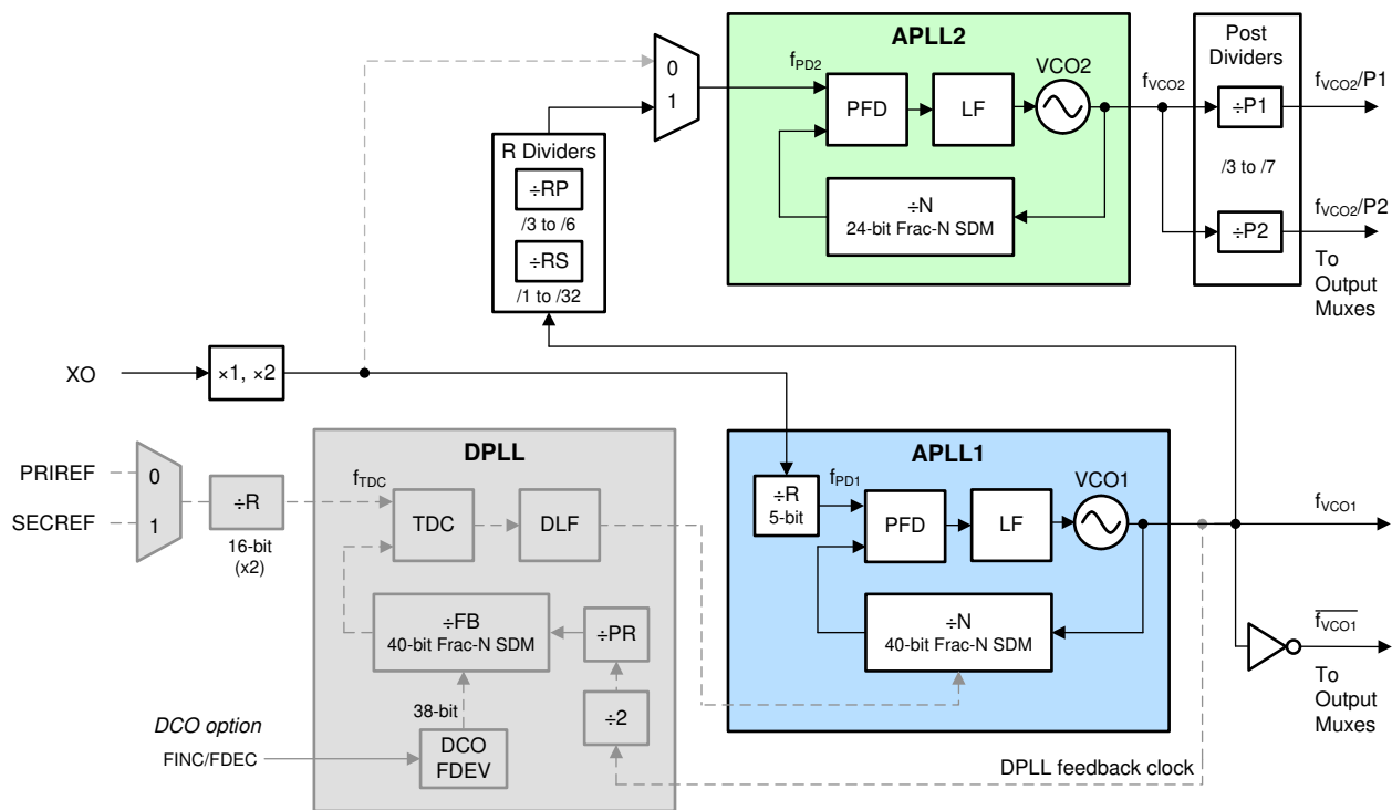
図 7-5. APLL-Only Mode With Cascaded APLL2
