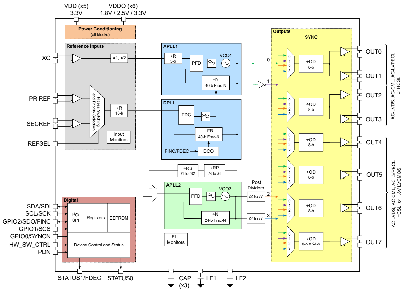
图 7-1. Top-Level Device Block Diagram
