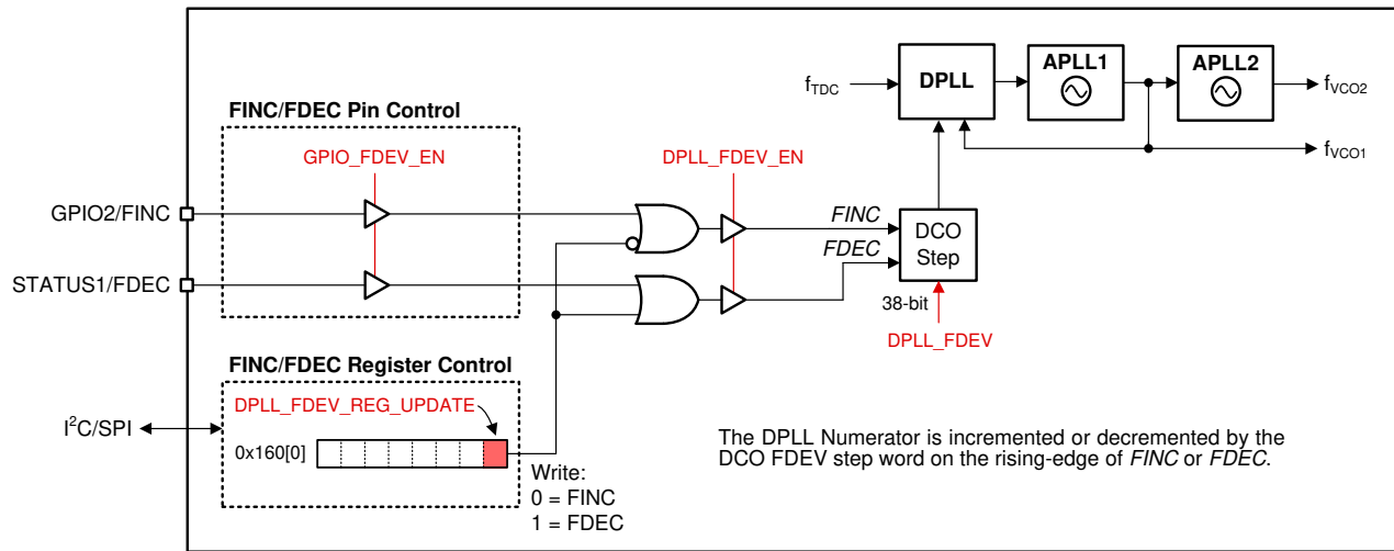
FIG 9-35. DCO Mode Control Options
