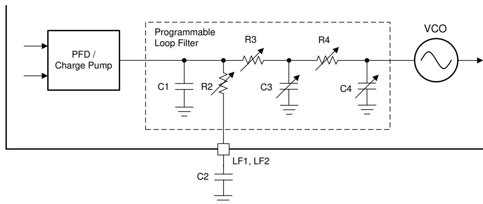
図 9-23. Loop Filter Structure of Each APLL
