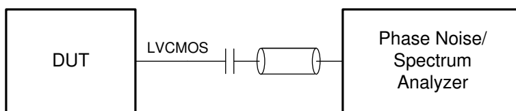
Figure 8-2. LVCMOS Output Phase Noise Test Configuration
