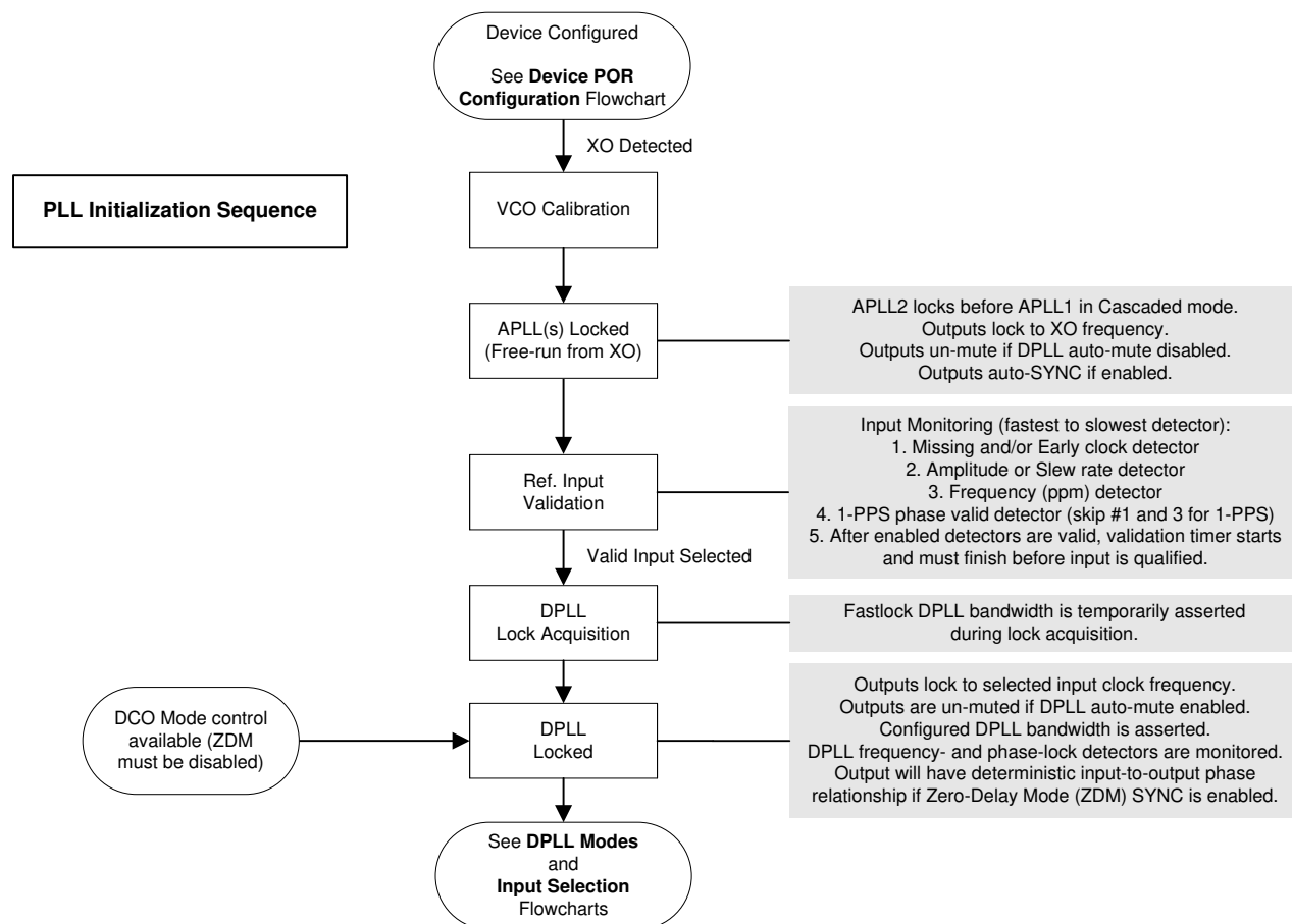
FIG 9-34. PLL Start-Up Sequence
