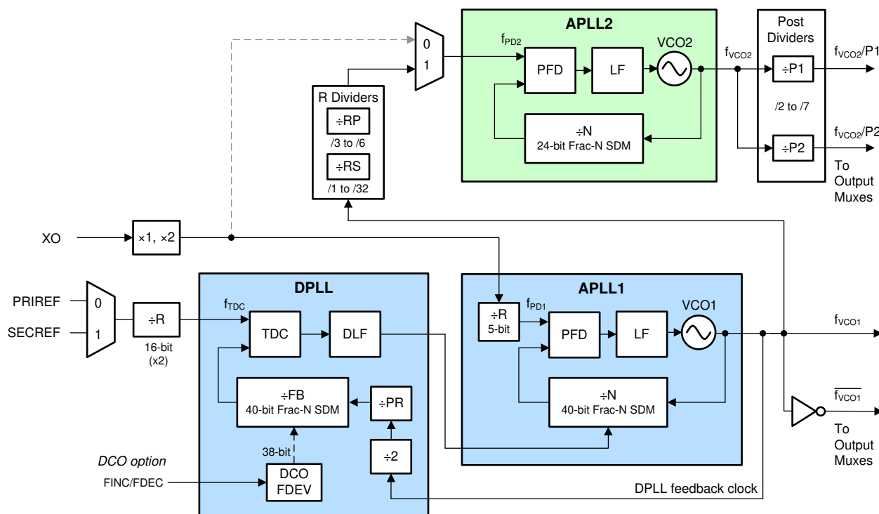
Figure 9-3. DPLL Mode With Cascaded APLL2
